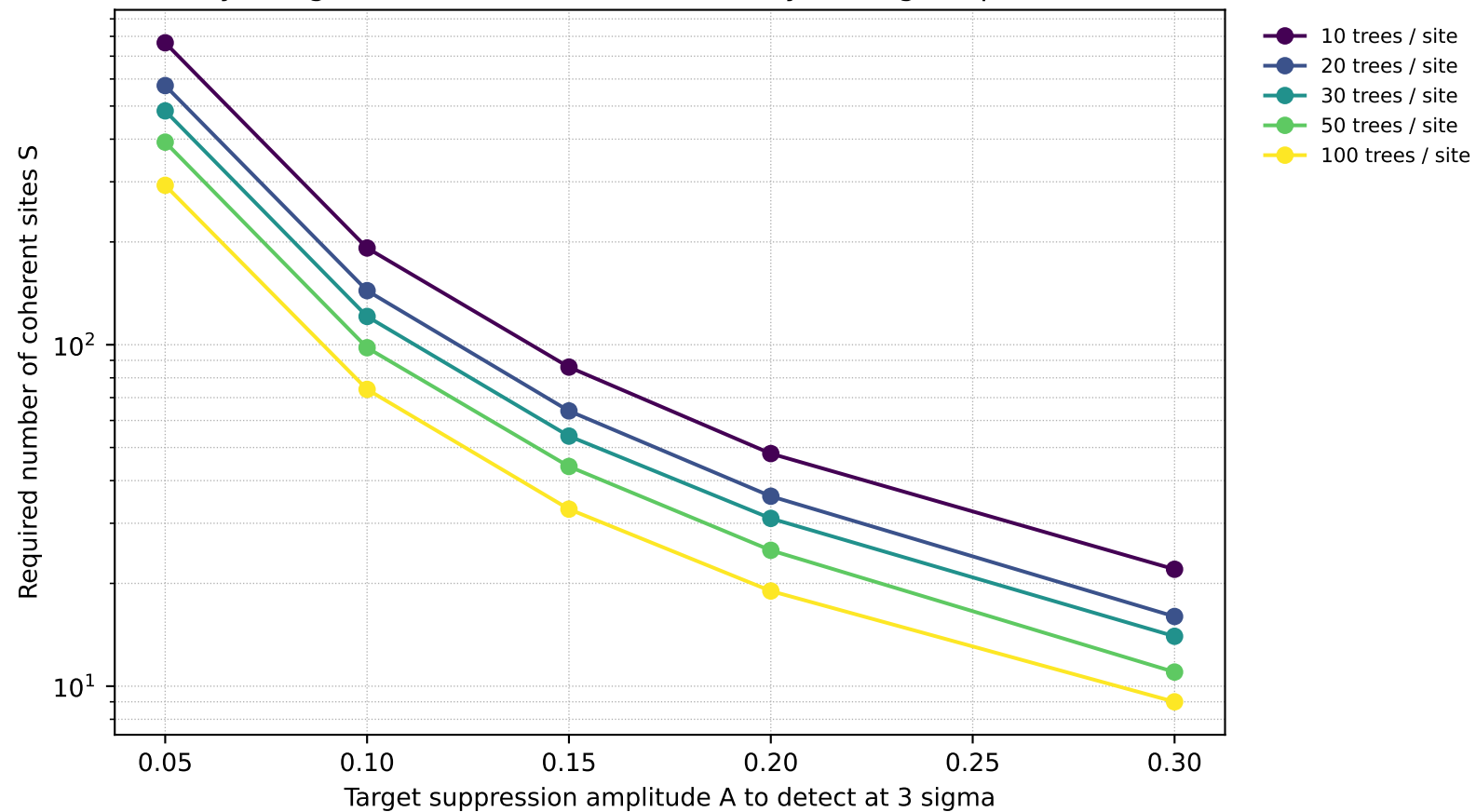
Array design from the measured sensitivity scaling (slope \sim n^{0.21} )
