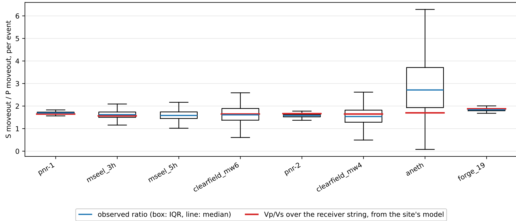
Observed moveout ratio against the velocity model's V_p/V_s
