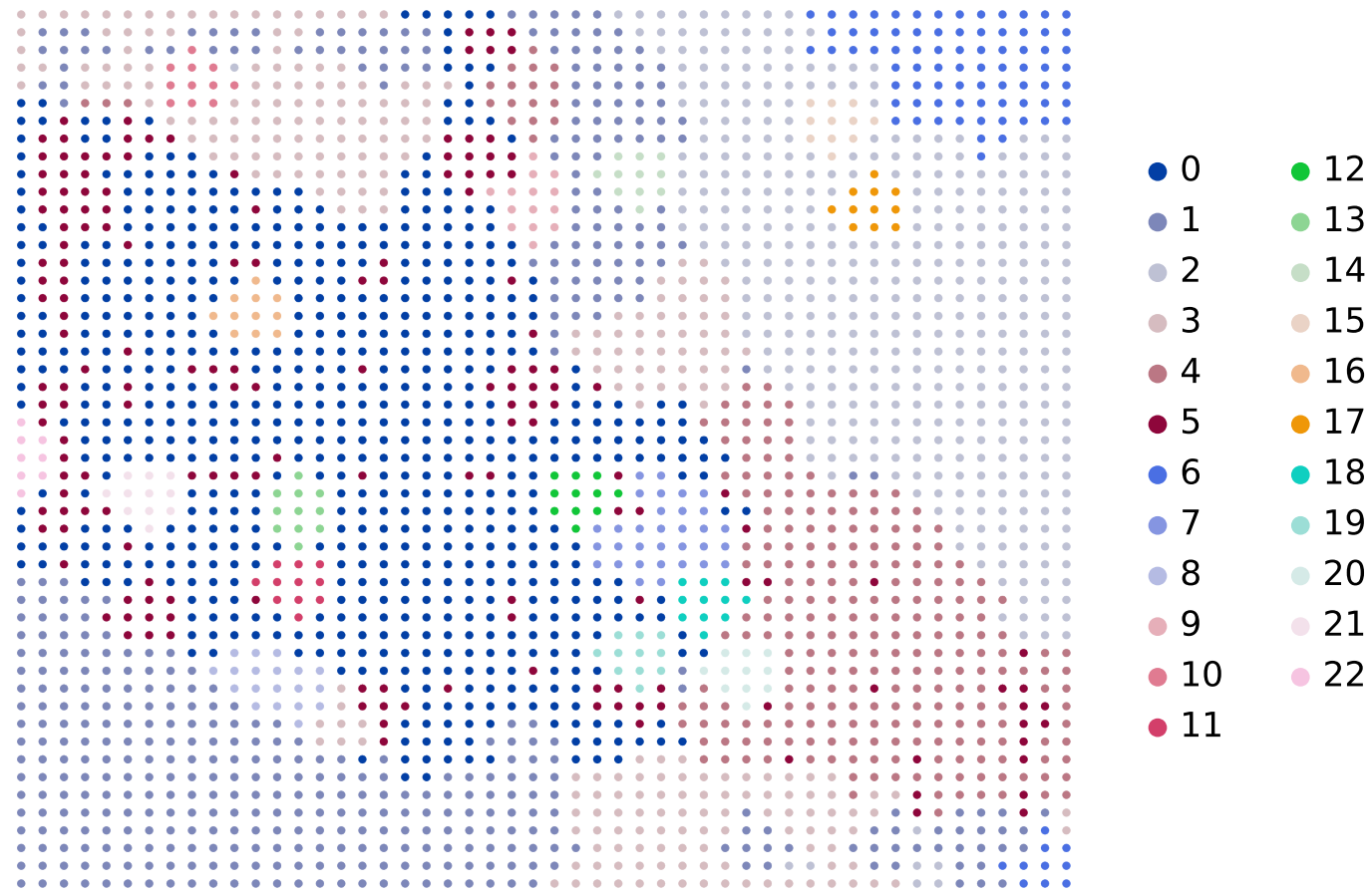
F_fre_rna (Spatial)
