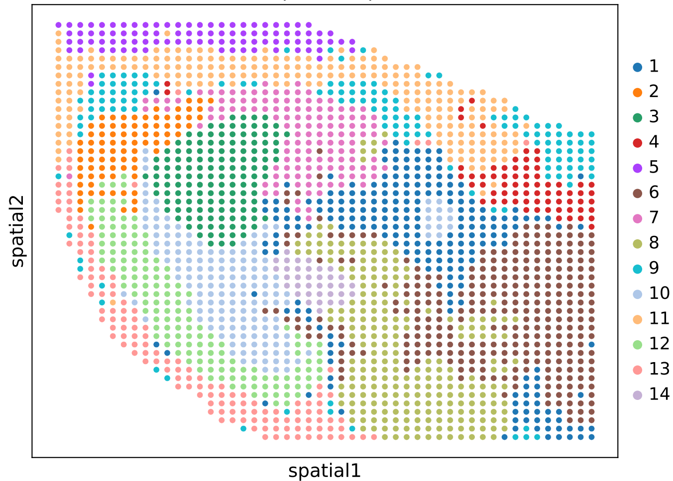
Spatial Map
