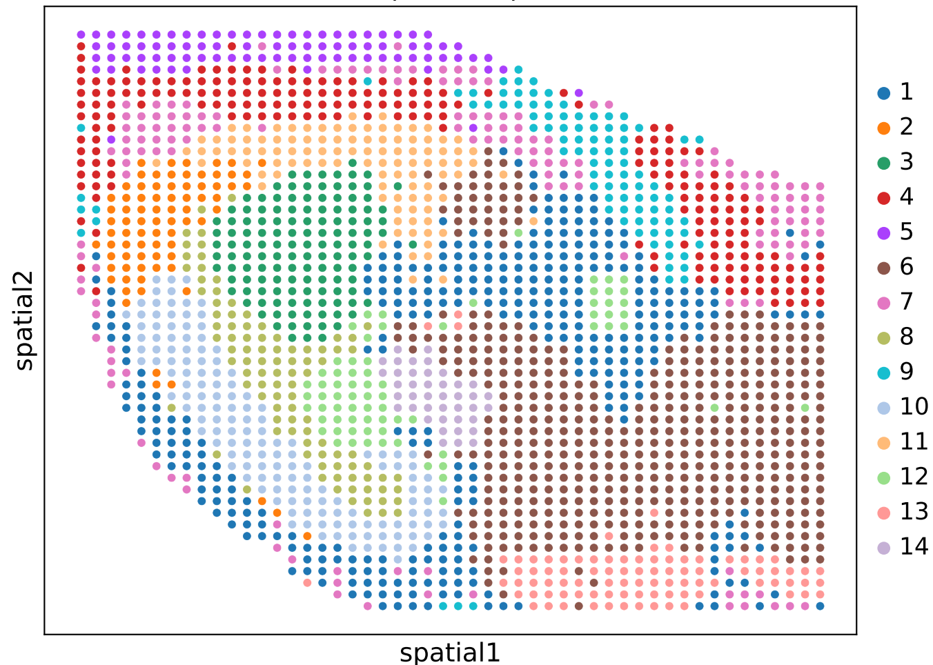
Spatial Map
