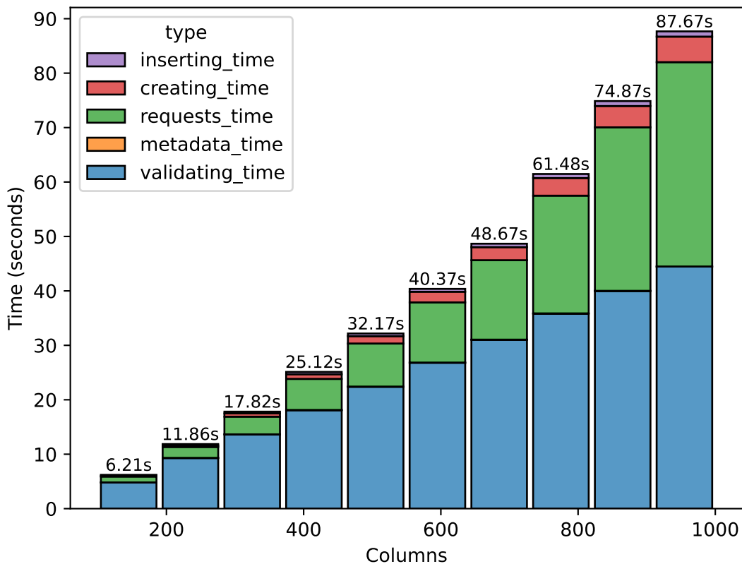
Full Execution Time (Fixed Rows: 1000; 20 iterations; 1 threads)
