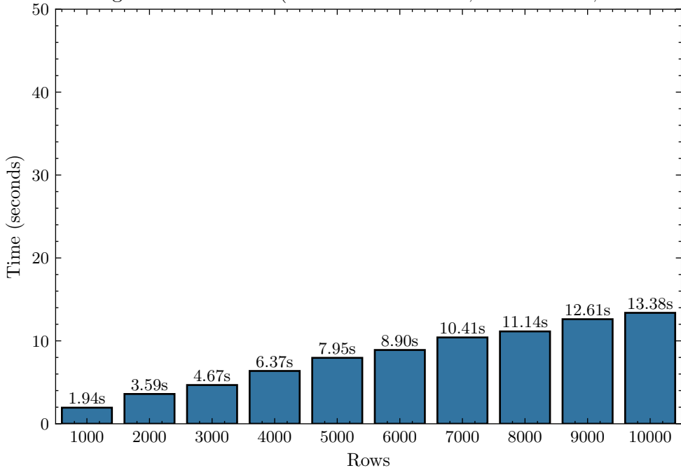
Validating Execution Time (Fixed Columns: 100; 20 iterations; 16 threads)
