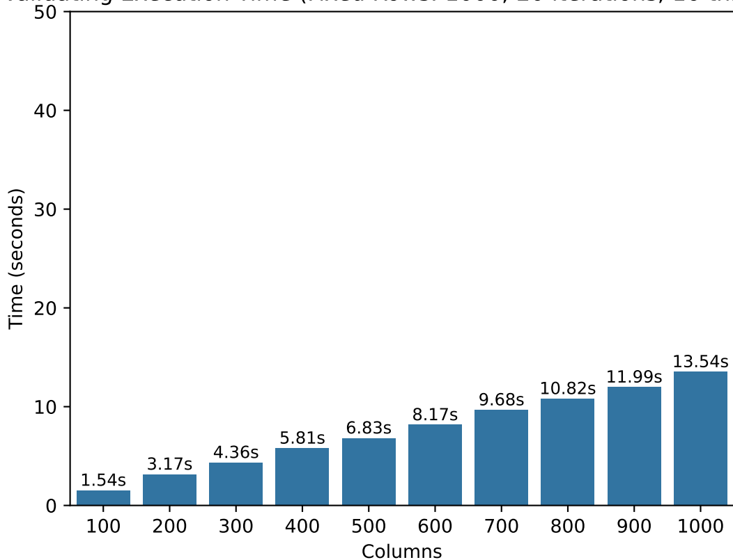
Validating Execution Time (Fixed Rows: 1000; 20 iterations; 16 threads)
