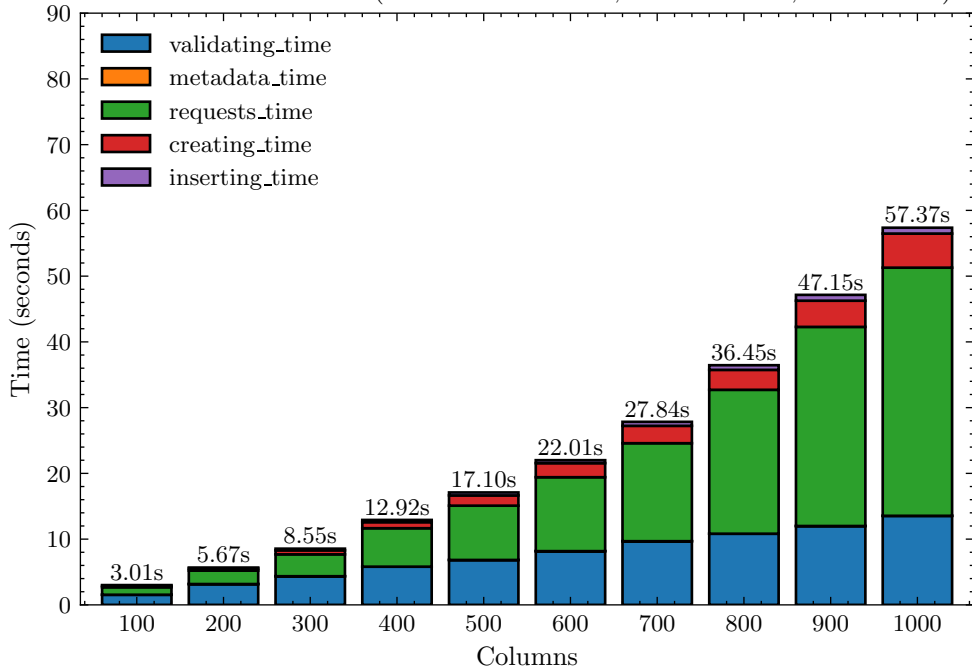
Full Execution Time (Fixed Rows: 1000; 20 iterations; 16 threads)
