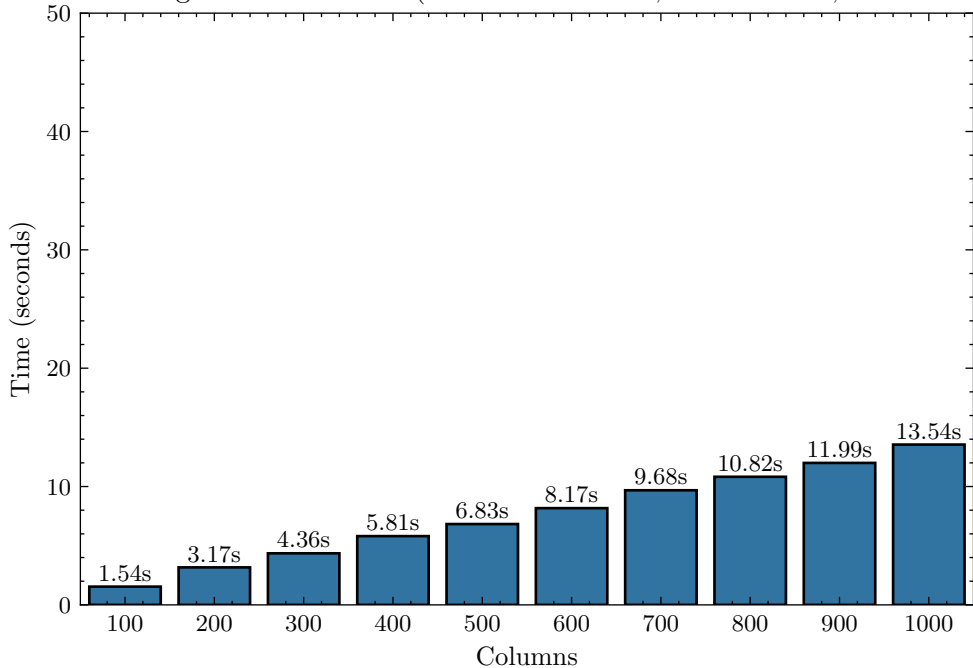
Validating Execution Time (Fixed Rows: 1000; 20 iterations; 16 threads)
