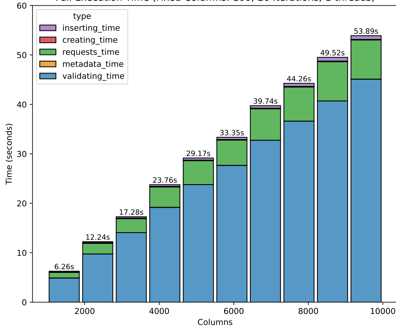
Full Execution Time (Fixed Columns: 100; 20 iterations; 1 threads)
