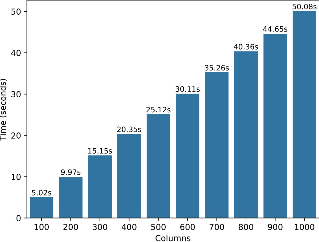
Validating Execution Time (Fixed Rows: 1000; 20 iterations; 1 threads)
