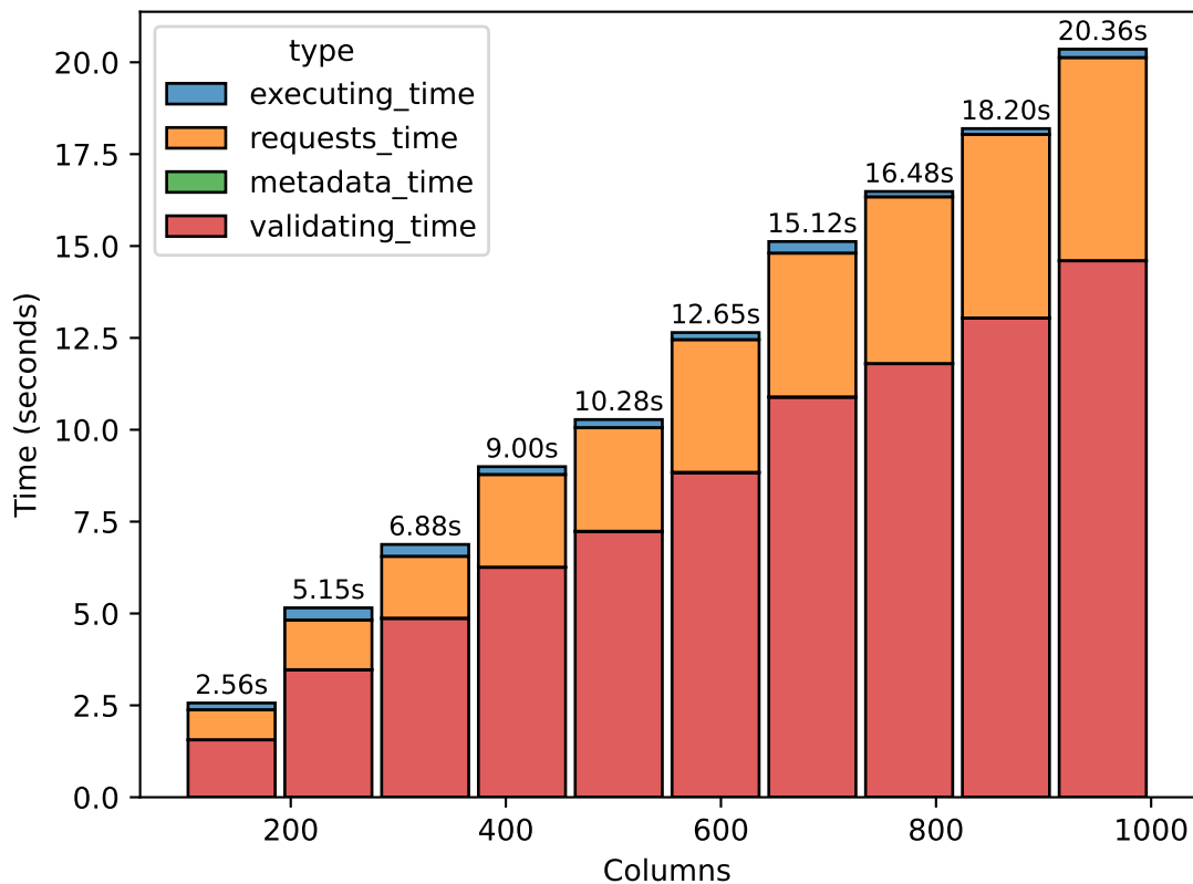
Full Execution Time (Fixed Rows: 1000; 20 iterations; 16 threads)
