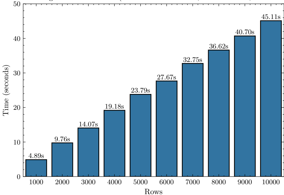
Validating Execution Time (Fixed Columns: 100; 20 iterations; 1 threads)
