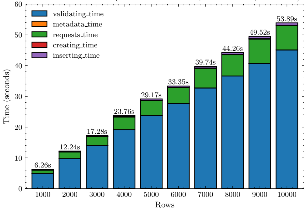
Full Execution Time (Fixed Columns: 100; 20 iterations; 1 threads)
