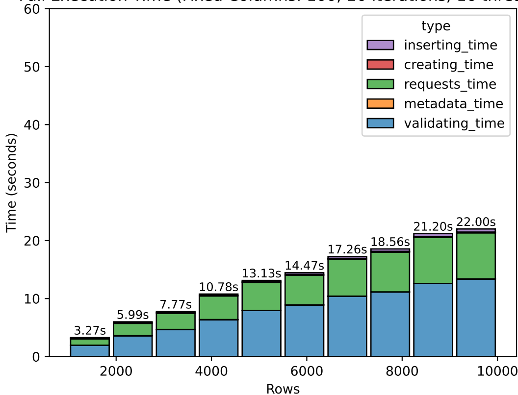
Full Execution Time (Fixed Columns: 100; 20 iterations; 16 threads)
