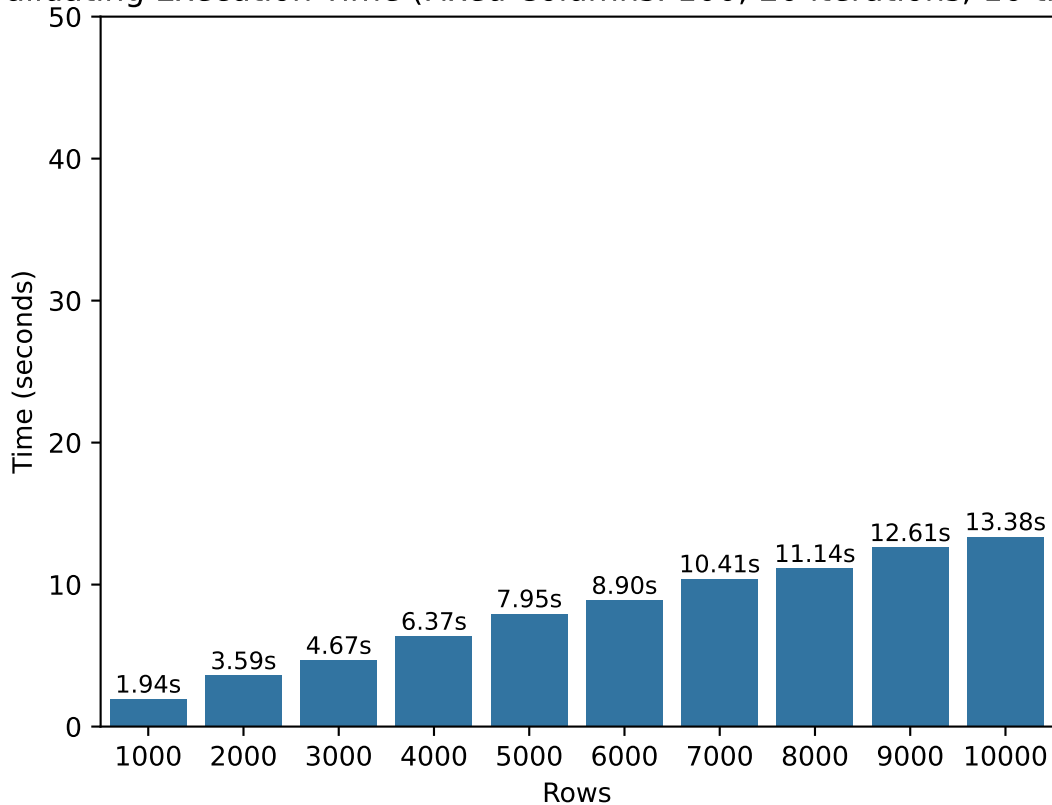
Validating Execution Time (Fixed Columns: 100; 20 iterations; 16 threads)
