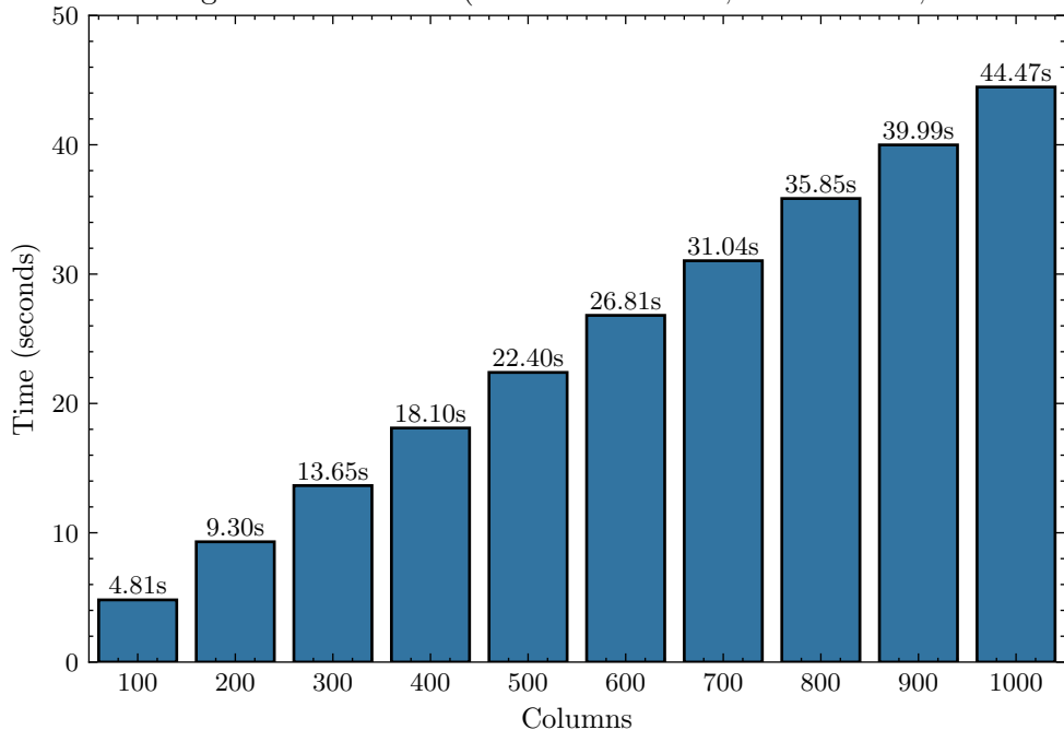
Validating Execution Time (Fixed Rows: 1000; 20 iterations; 1 threads)
