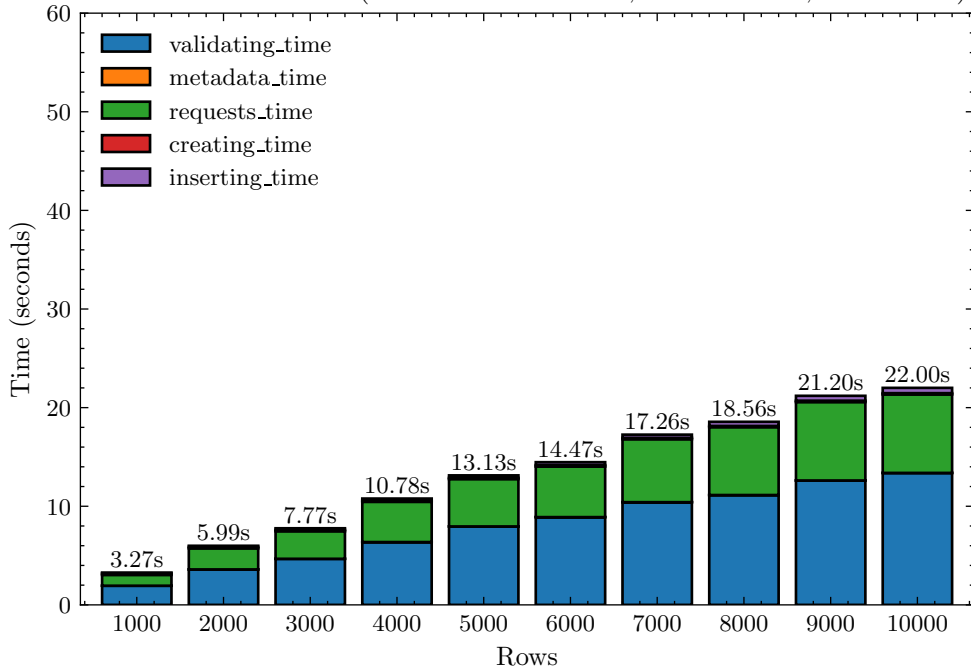
Full Execution Time (Fixed Columns: 100; 20 iterations; 16 threads)
