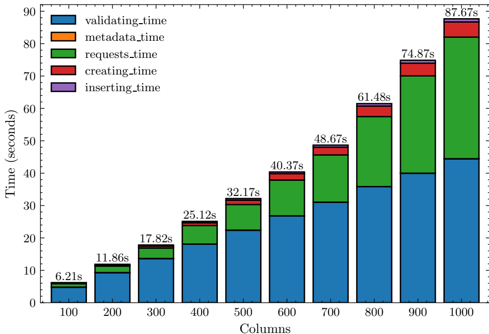
Full Execution Time (Fixed Rows: 1000; 20 iterations; 1 threads)
