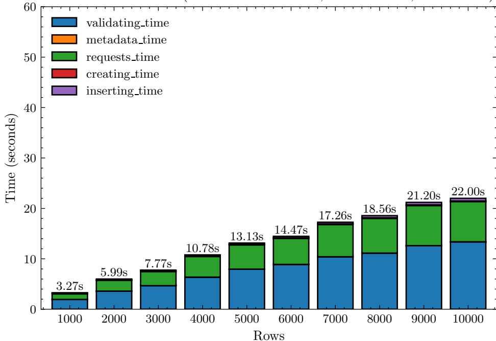
Full Execution Time (Fixed Columns: 100; 20 iterations; 16 workers)
