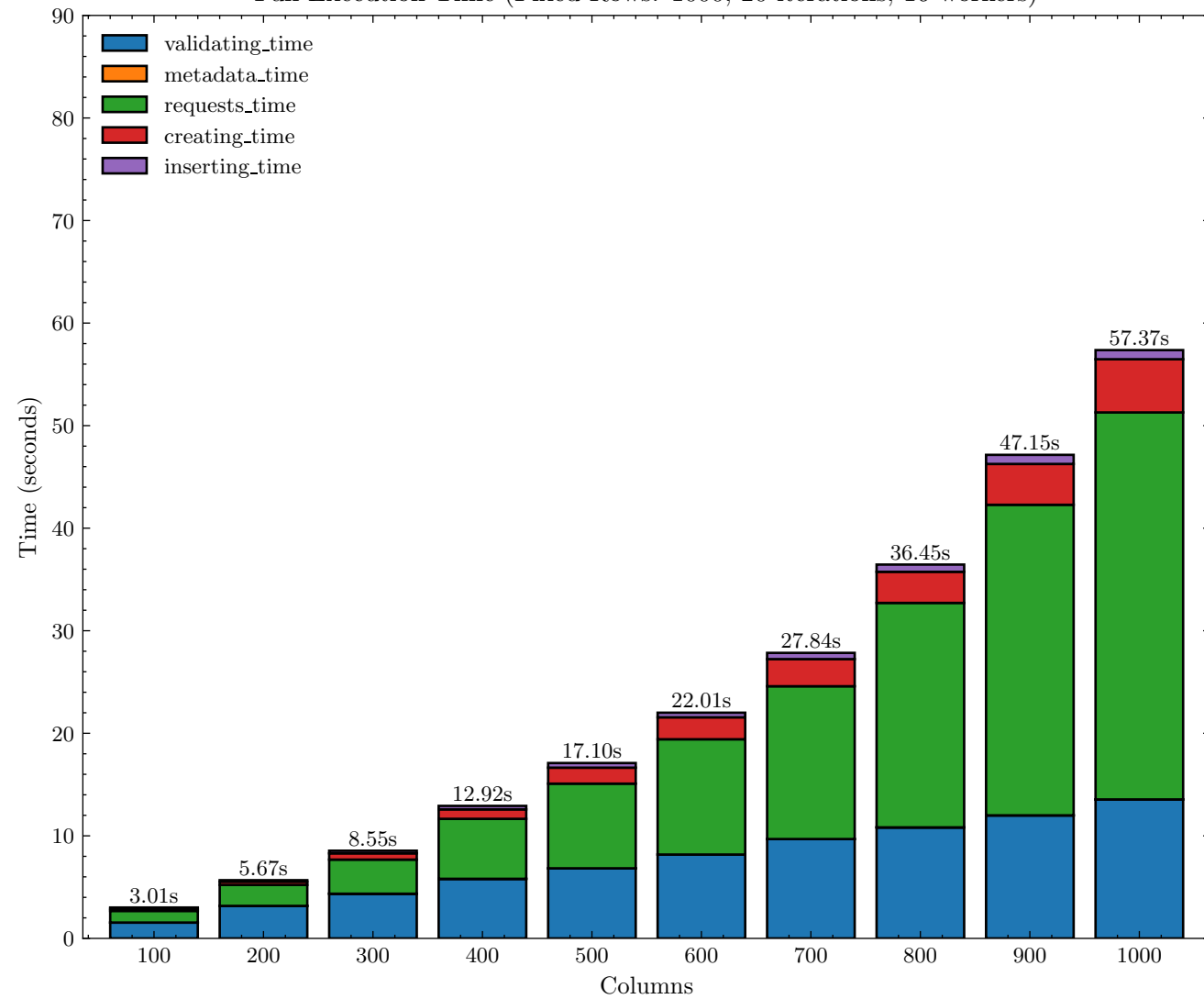
Full Execution Time (Fixed Rows: 1000; 20 iterations; 16 workers)
