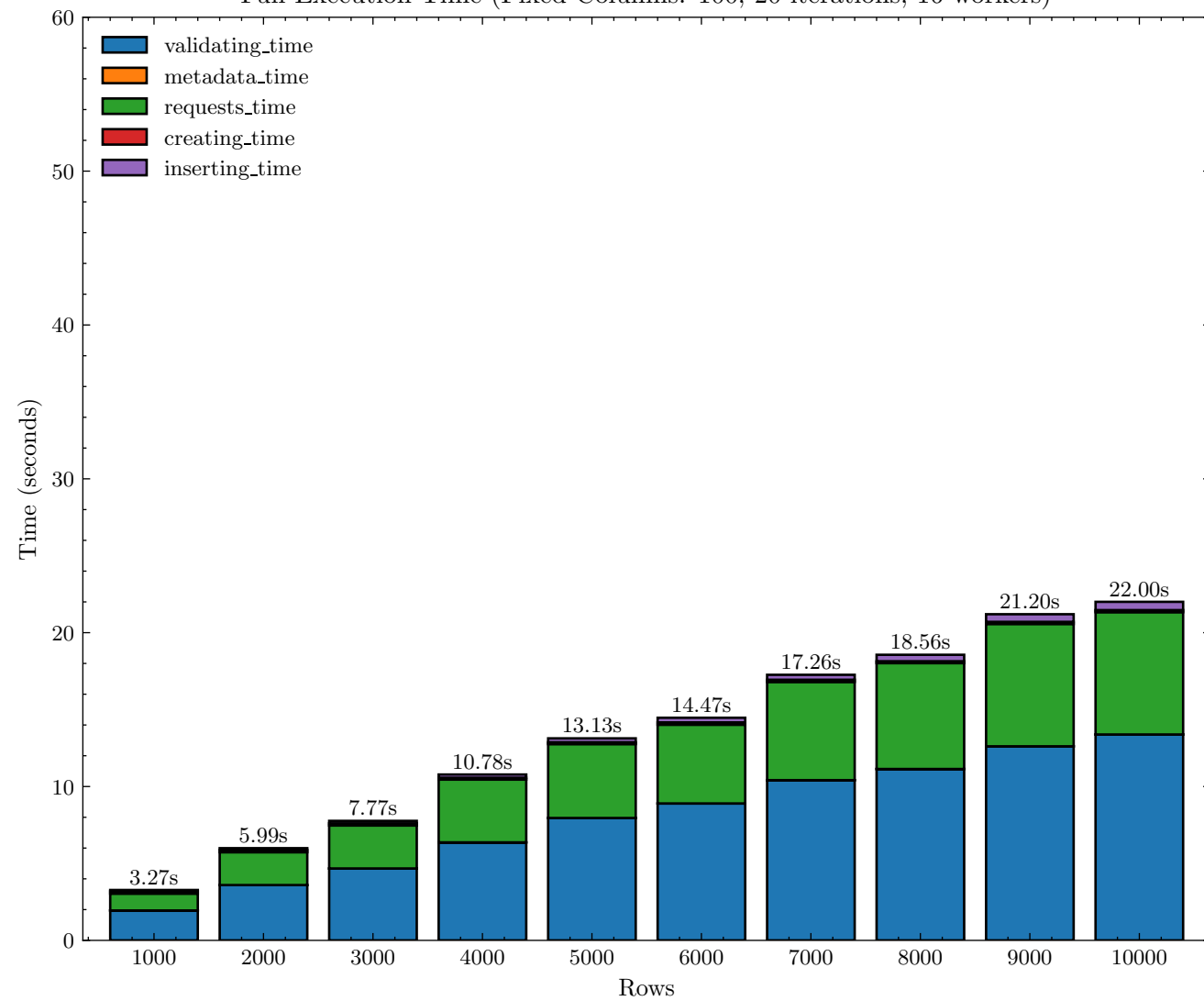
Full Execution Time (Fixed Columns: 100; 20 iterations; 16 workers)
