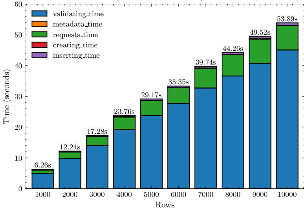
Full Execution Time (Fixed Columns: 100; 20 iterations; 1 worker)
