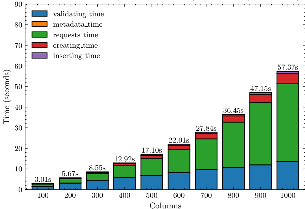
Full Execution Time (Fixed Rows: 1000; 20 iterations; 16 workers)
