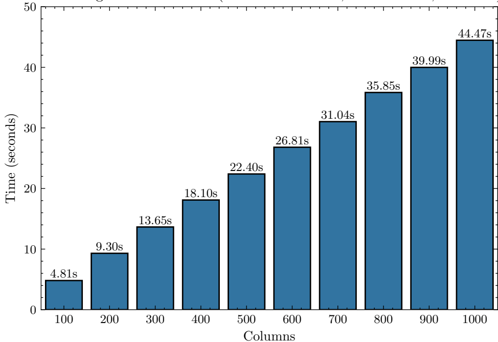
Validating Execution Time (Fixed Rows: 1000; 20 iterations; 1 worker)
