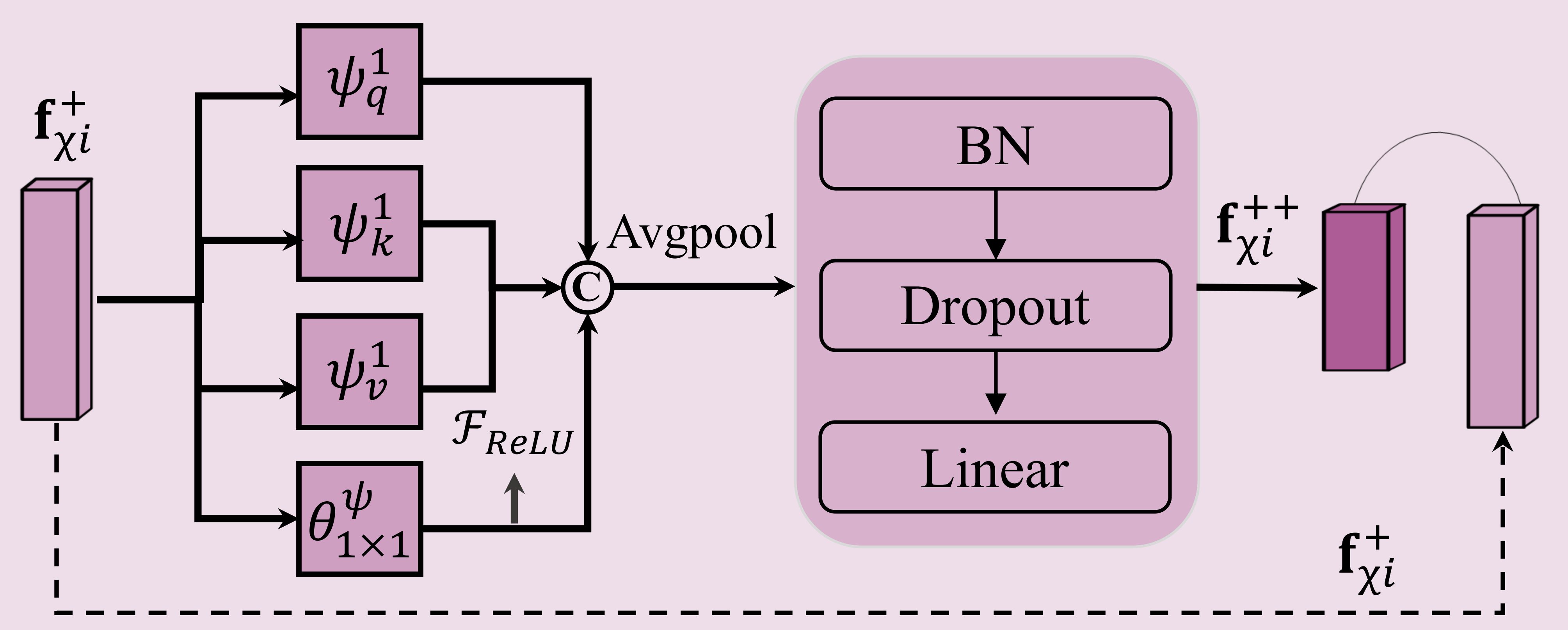
Diversified Embedding Classifier (DEC)
