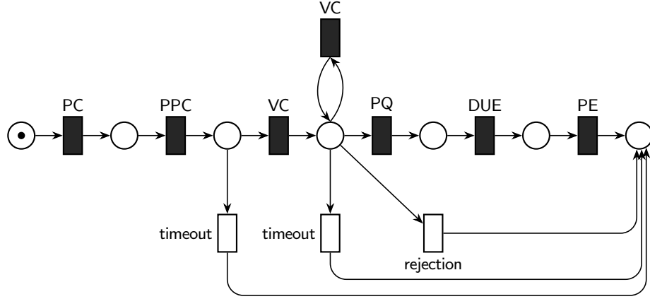
Fig. 4. Reference Petri net of the on-chain deployment lifecycle. Filled transitions correspond to on-chain events: PC = ProposalCreated, PPC = ProposalPackageCreated, VC = VoteCast, PQ = ProposalQueued, DUE = DeterministicUpgradeExecuted, PE = ProposalExecuted, the final event in (C1) in Table 3. Unfilled transitions are silent: rejection models a negative quorum (C2) in Table 3, requiring at least 1 vote; timeout models an expired voting period without majority (C3) in Table 3, which can happen with 0 or more votes. Initial marking: p_0 ; final marking: p_6 .
