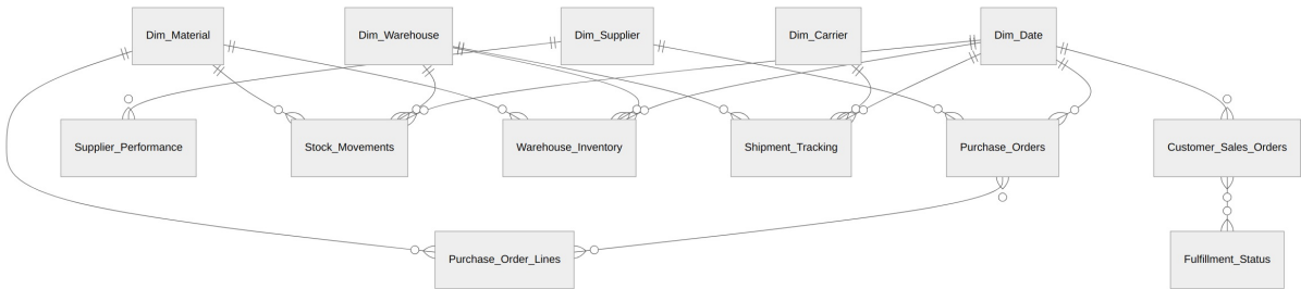
Model Relationship Diagram
