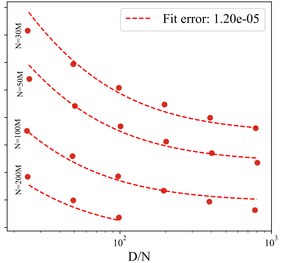
\beta = 1 Model, Kaplan et al.
