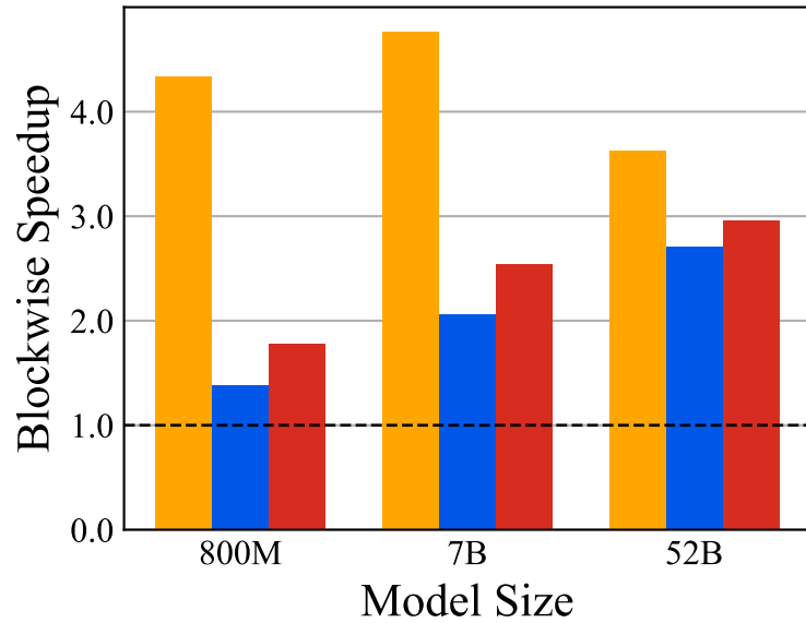
MXFP4 vs BF16 Speedup
