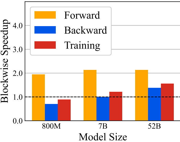
MXFP4 vs FP8 Speedup
