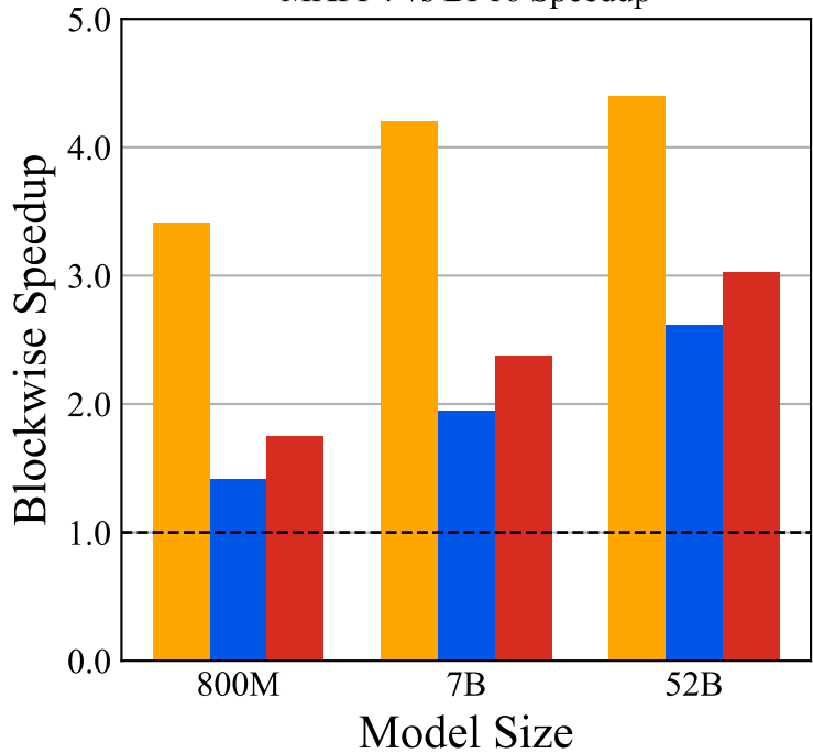
MXFP4 vs BF16 Speedup
