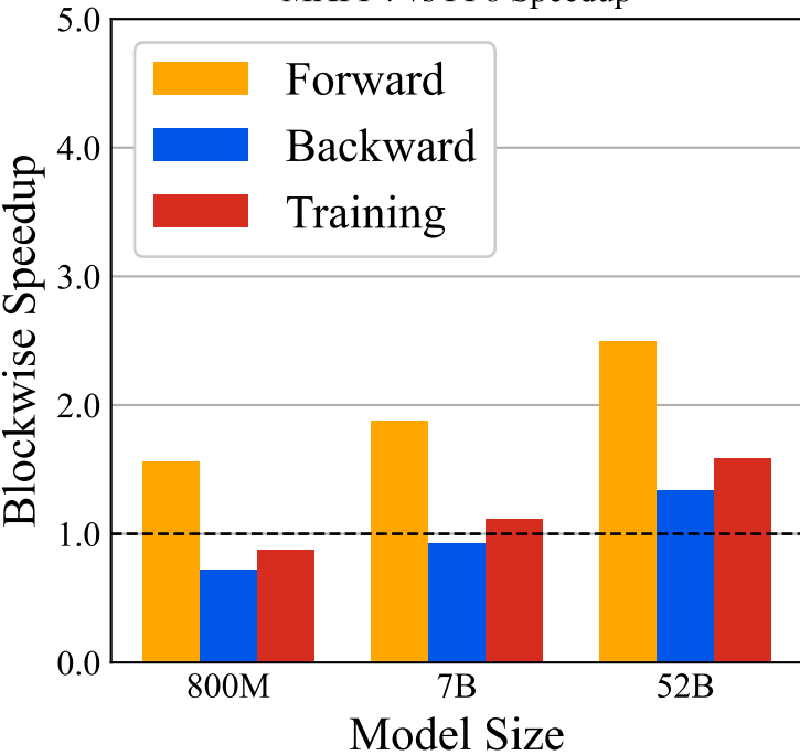
MXFP4 vs FP8 Speedup
