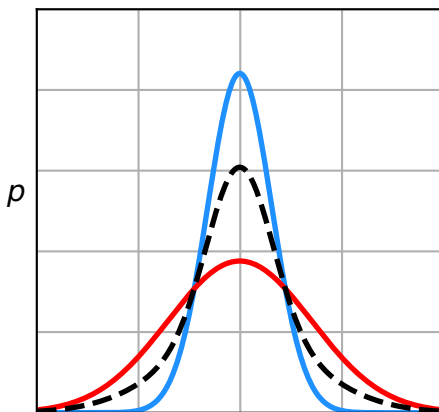
Marginal Distribution (Original)
