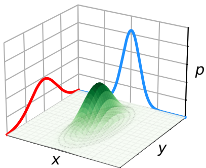
Joint Distribution (Original)
