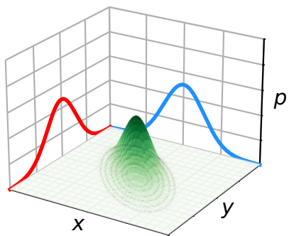
Joint Distribution (Rotated)
