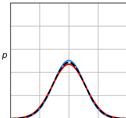
Marginal Distribution (Rotated)
