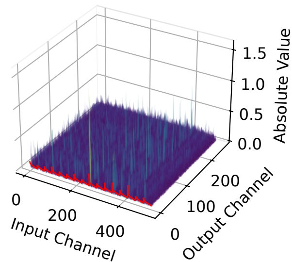
Activation - WUS
