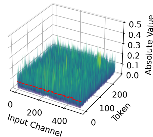
Activation - WUSH
