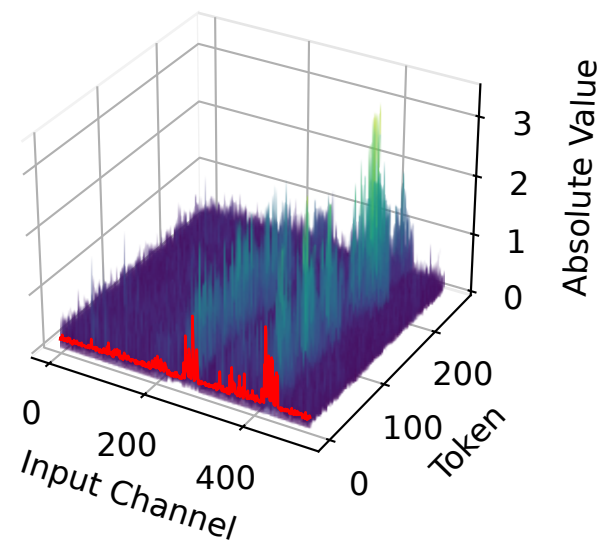
Activation - R
