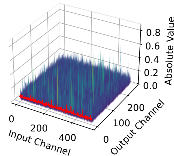
Activation - SmoothQuant
