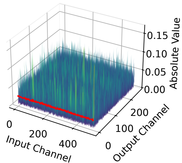
Activation - H
