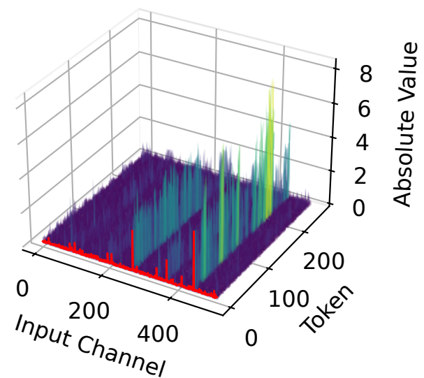
Activation - I
