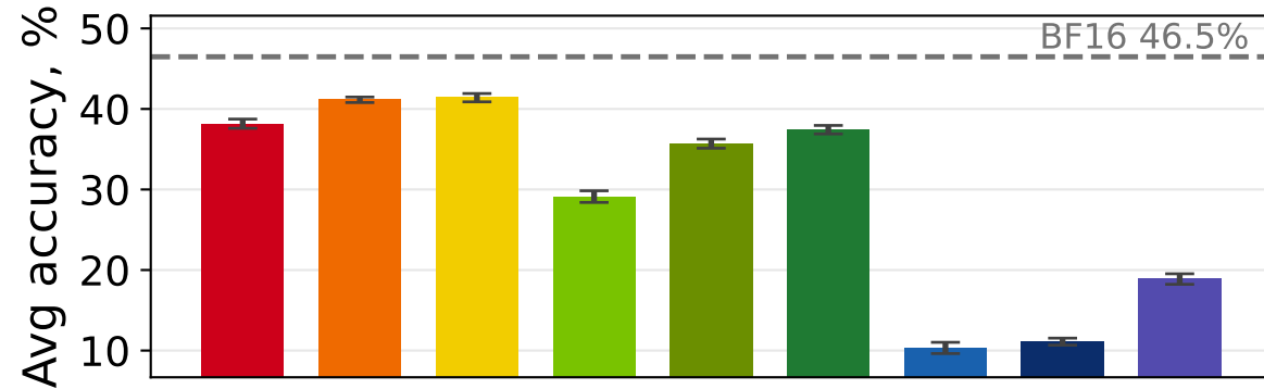
Qwen 3 8B
