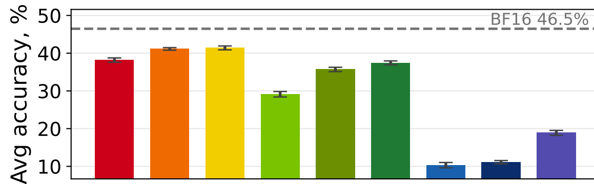
Qwen 3 8B
