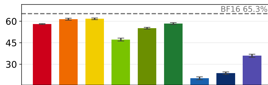
Qwen 3 1.7B
