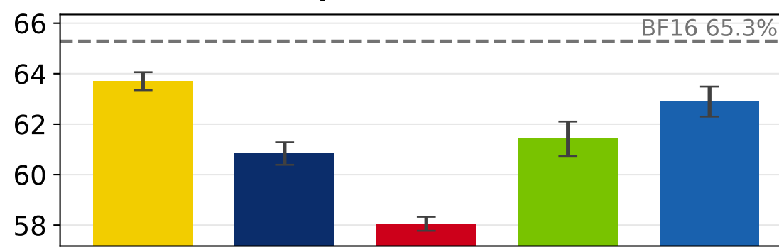
Qwen 3 1.7B
