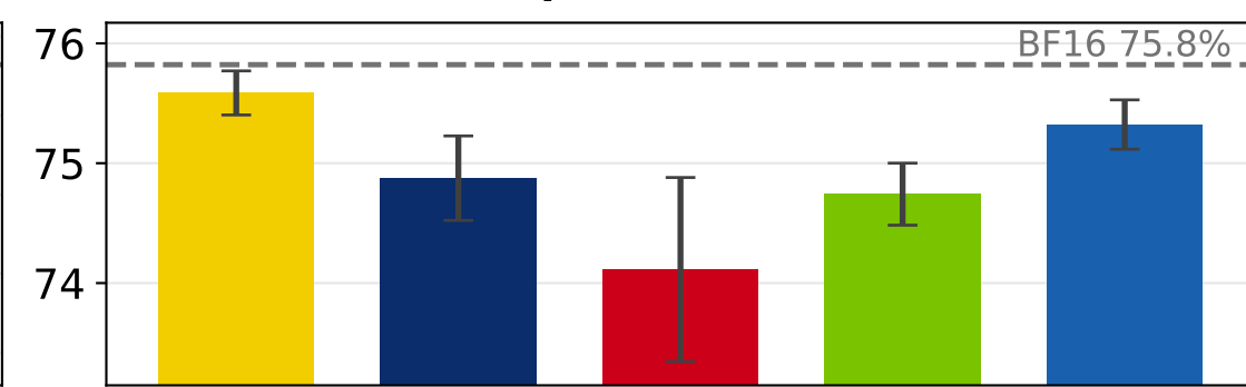
Qwen 3 4B
