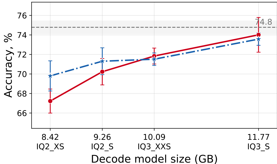
MMMUPro (vision)
