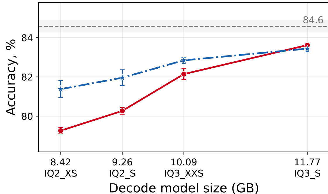
MMLU-Pro
