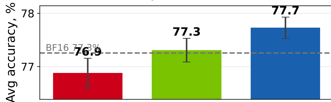
Qwen 3 8B
