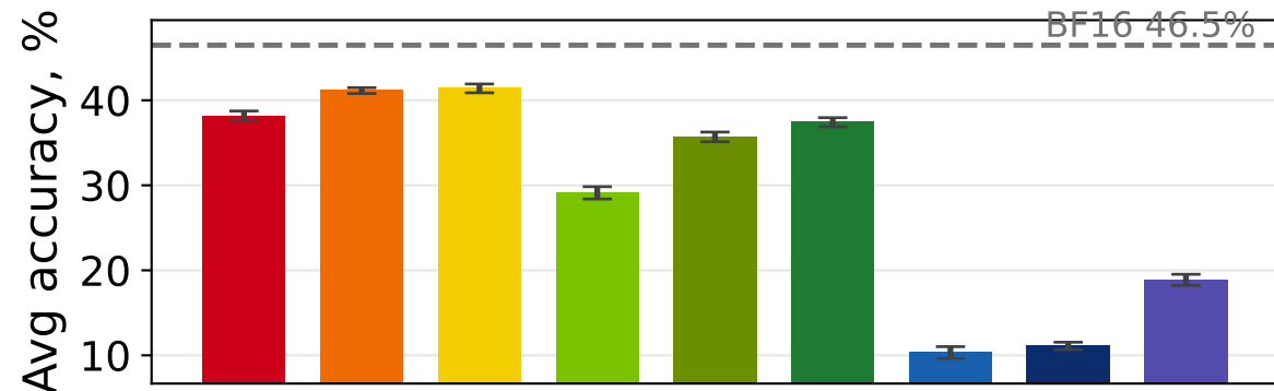
Qwen 3 8B
