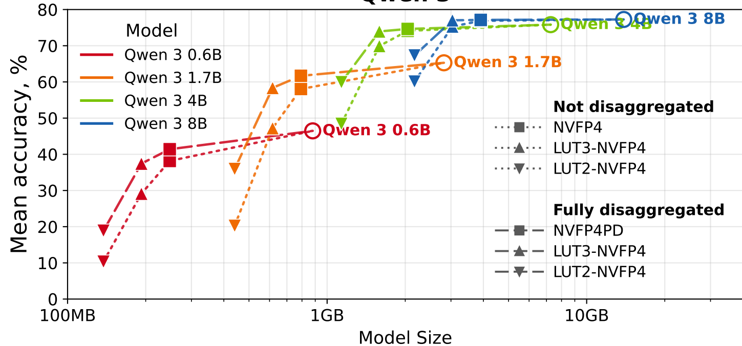
Qwen 3
