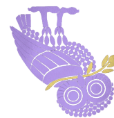
METACOGNITIVE
