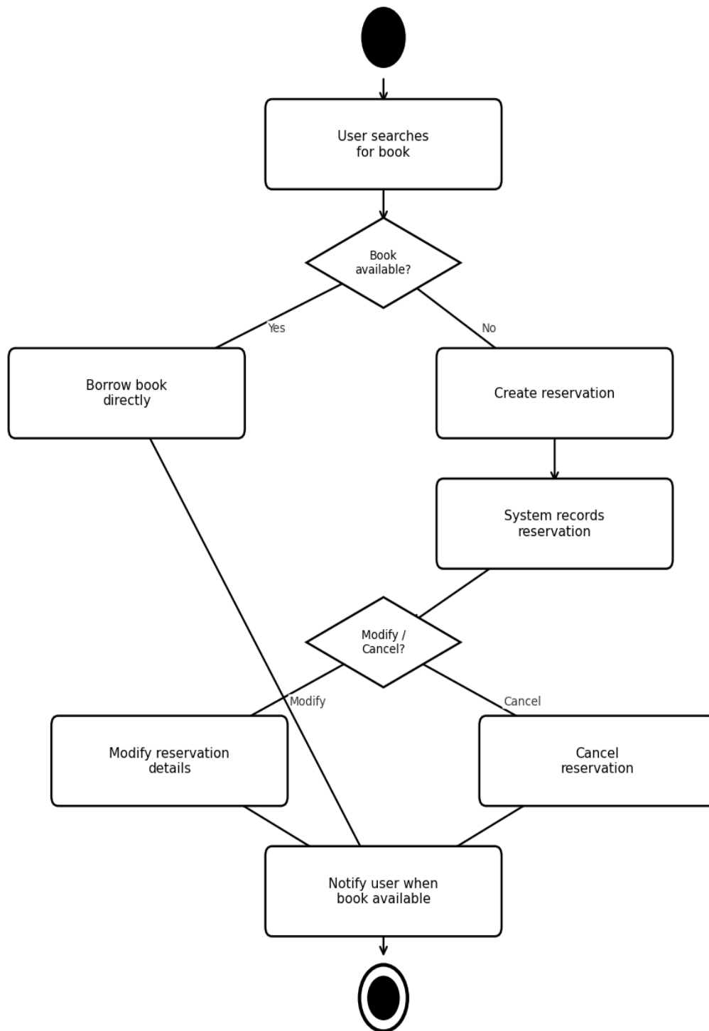
Reservation Management - Activity Diagram
