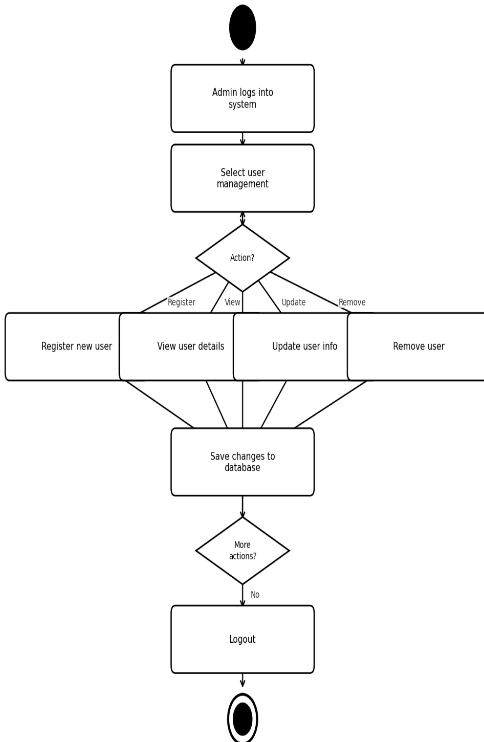
User Management - Activity Diagram
