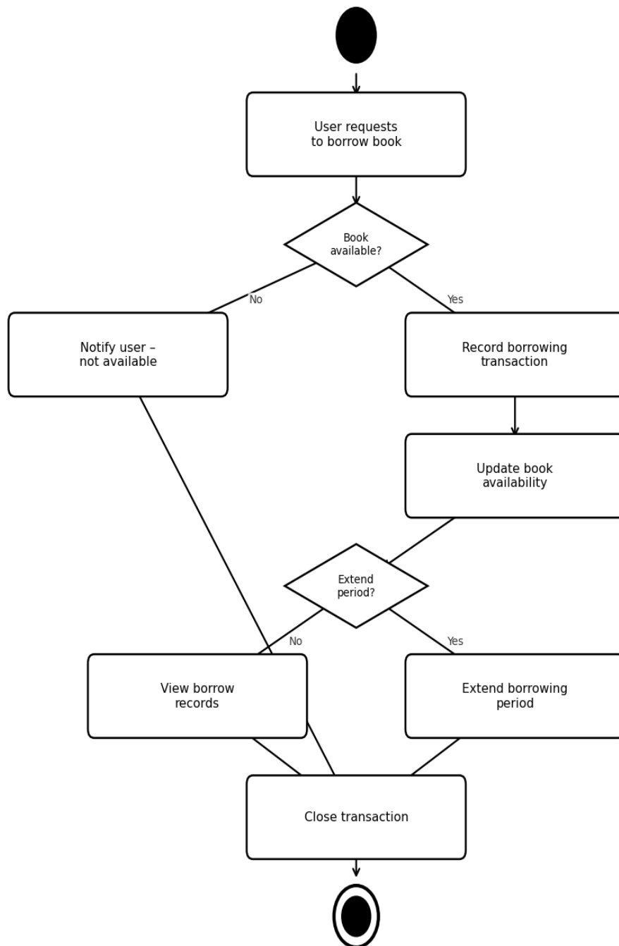
Borrowing Management - Activity Diagram
