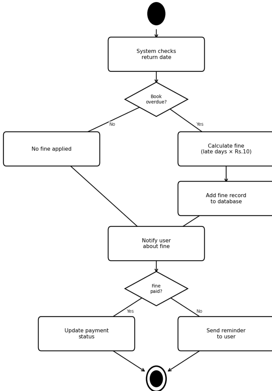
Fine Management - Activity Diagram
