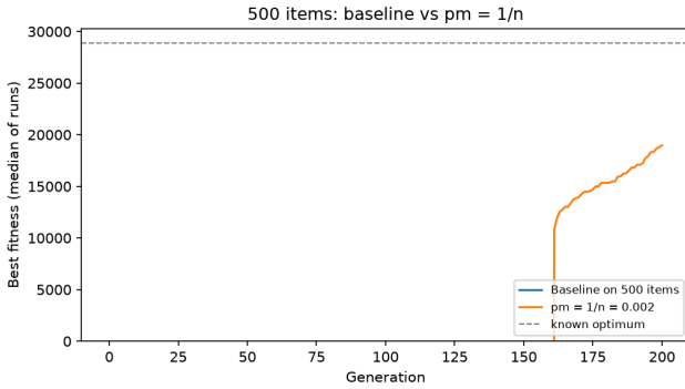
Figure 5: 500 items: median best fitness over 10 runs.
