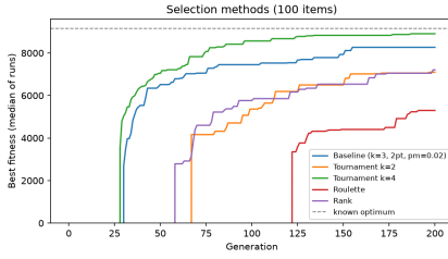
Figure 2: Selection.
