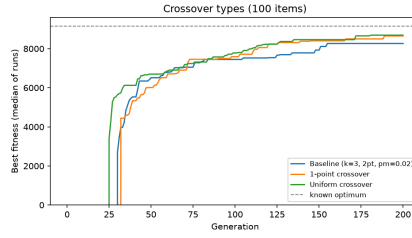
Figure 3: Crossover.
