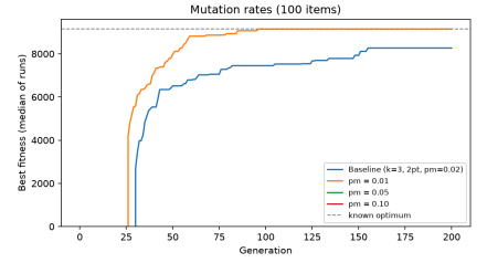
Figure 4: Mutation rate.
