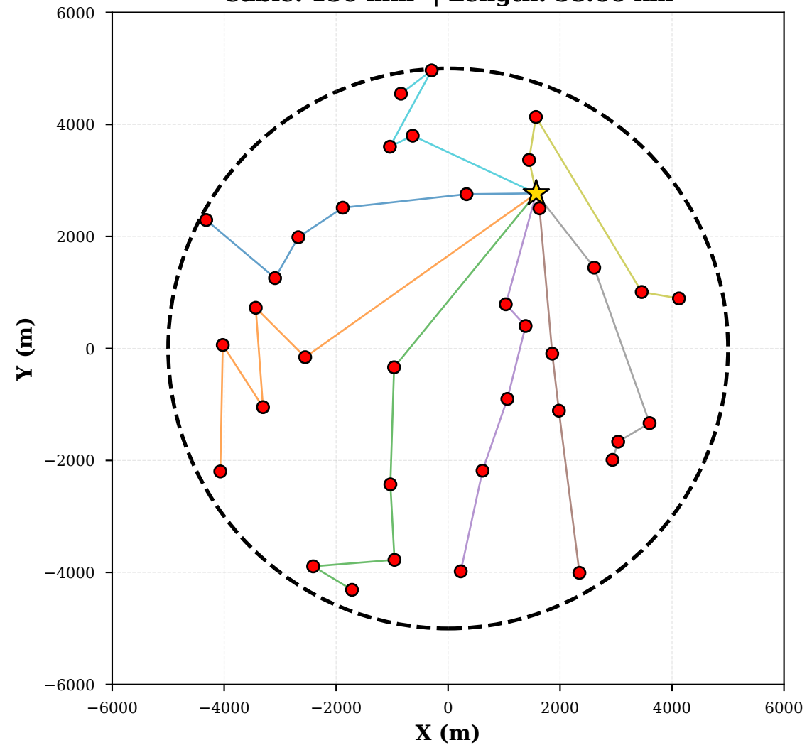
Phase 2 - Knee Point AEP: 937.83 GWh | Cost: $1580k USD Cable: 150 mm 2 | Length: 58.66 km
