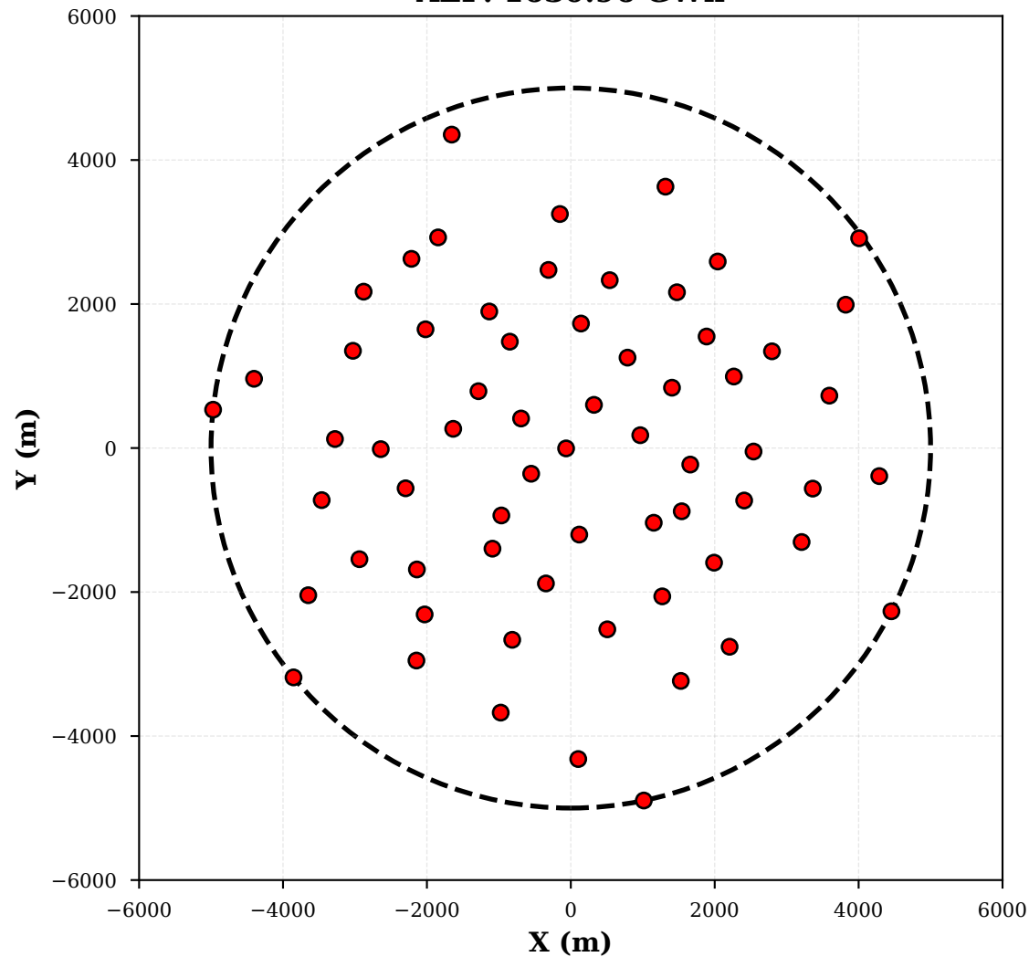
Phase 1 - Best AEP: 1630.96 GWh
