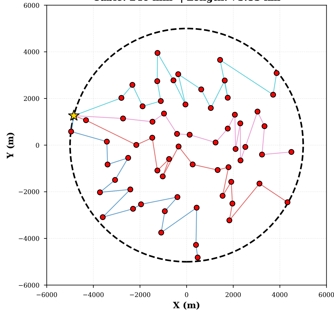
Phase 2 - Knee Point AEP: 1419.98 GWh | Cost: $3182k USD Cable: 240 mm 2 | Length: 73.83 km
