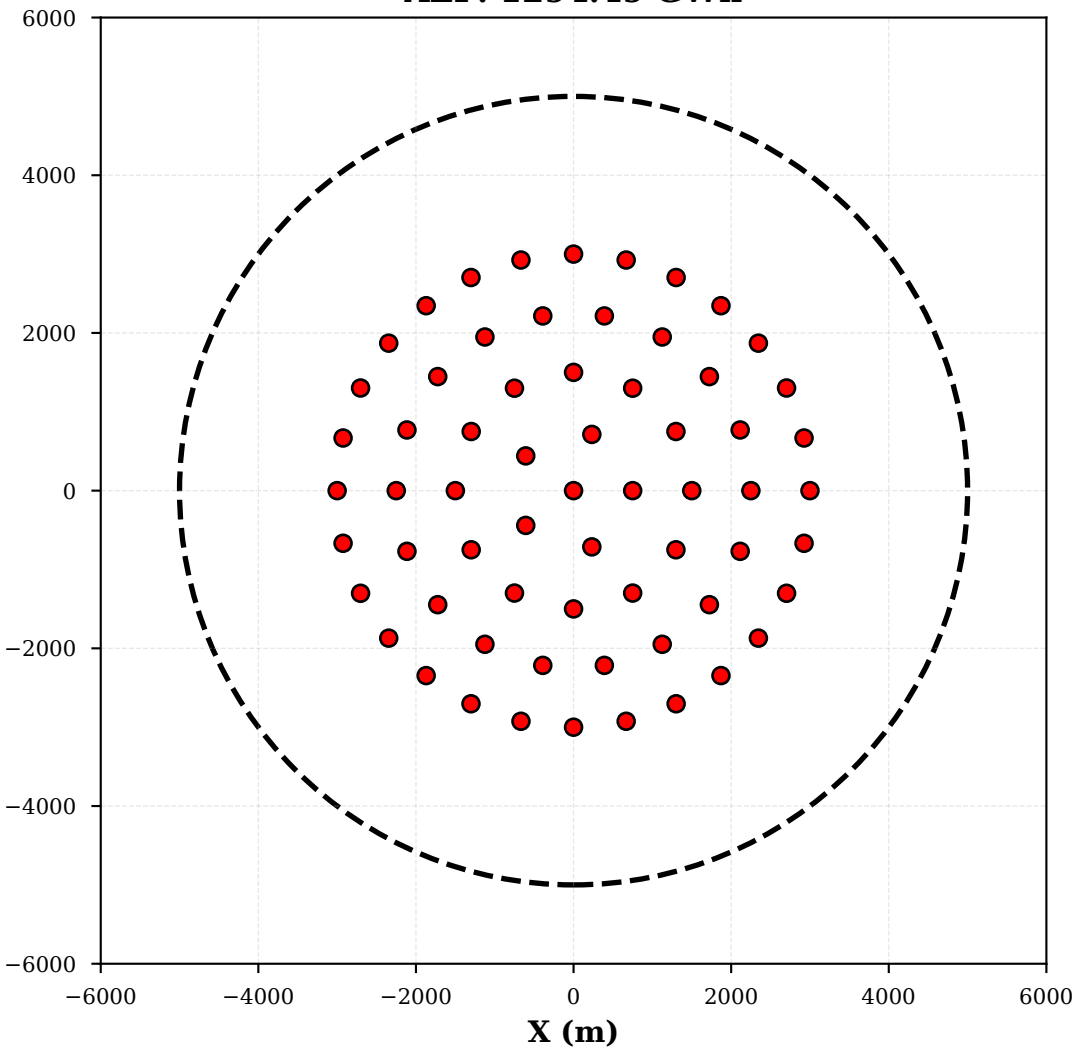
Phase 1 - Initial AEP: 1294.49 GWh
