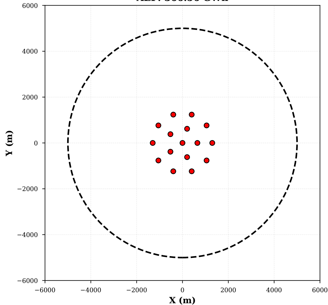
Phase 1 - Initial AEP: 366.56 GWh
