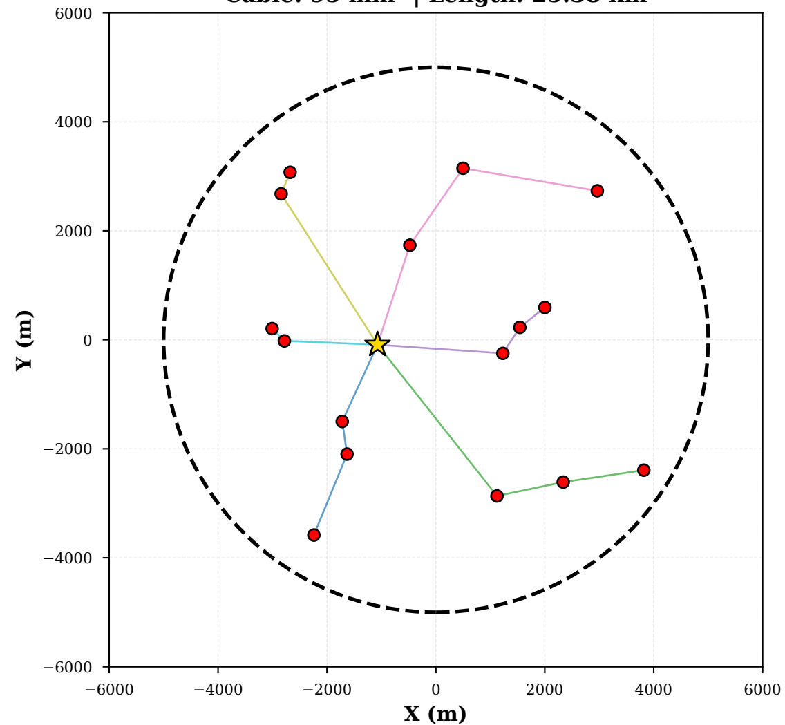
Phase 2 - Knee Point AEP: 441.36 GWh | Cost: $433k USD Cable: 95 mm 2 | Length: 25.38 km
