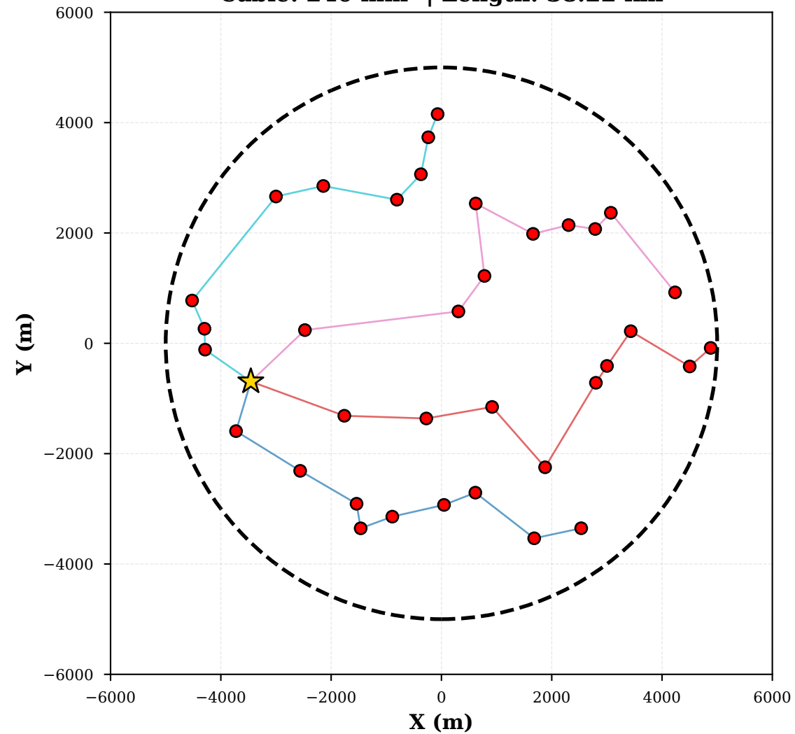
Phase 2 - Knee Point AEP: 916.31 GWh | Cost: $1647k USD Cable: 240 mm 2 | Length: 38.22 km
