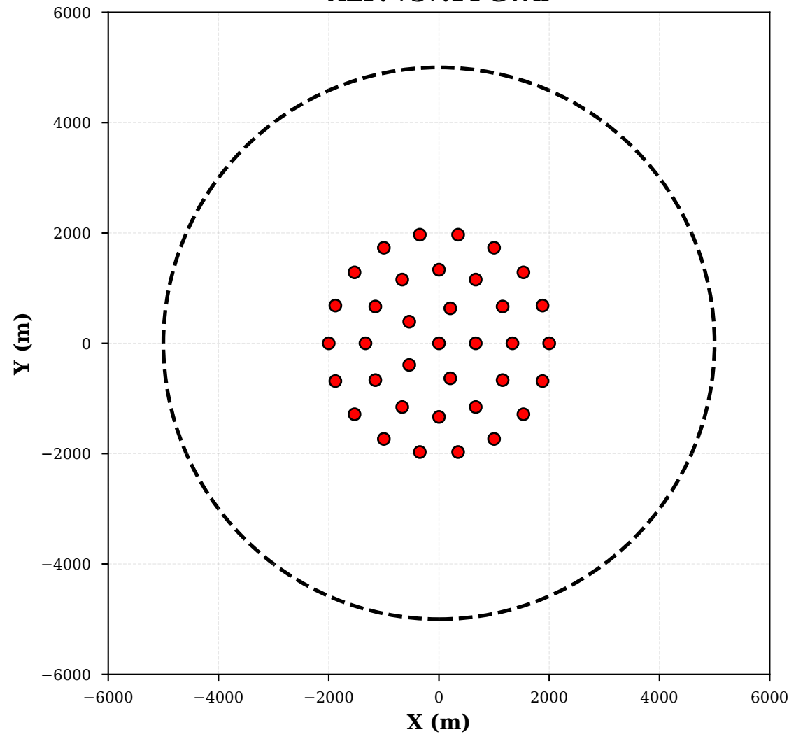
Phase 1 - Initial AEP: 737.14 GWh
