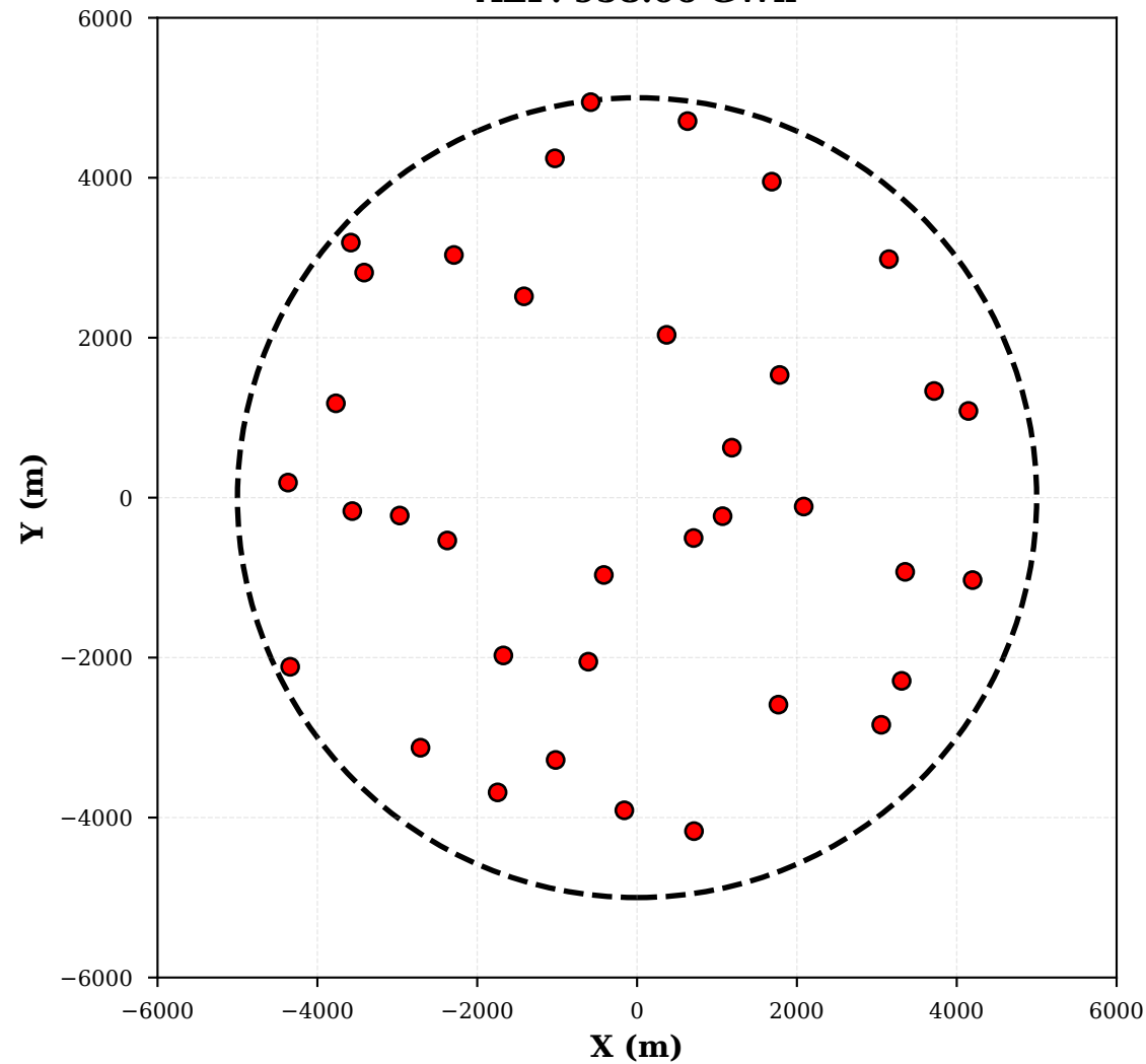
Phase 1 - Best AEP: 958.06 GWh
