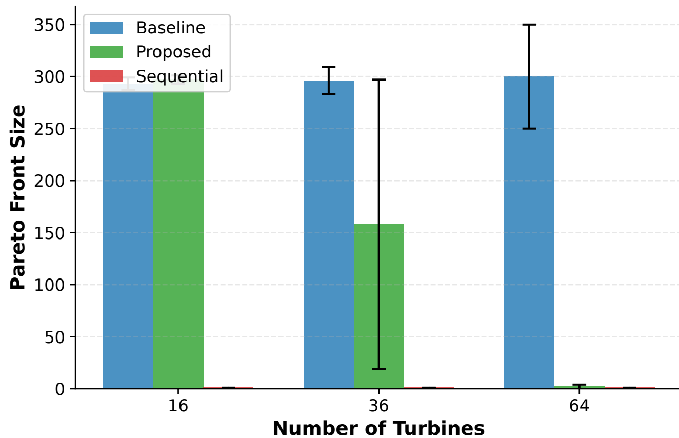
(a) Pareto Front Size
