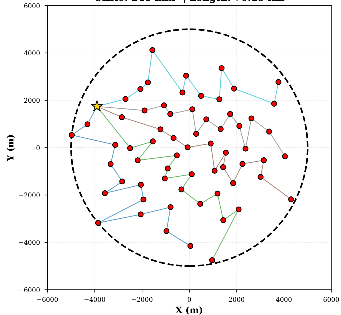
Phase 2 - Knee Point AEP: 1568.80 GWh | Cost: $3025k USD Cable: 240 mm 2 | Length: 70.19 km
