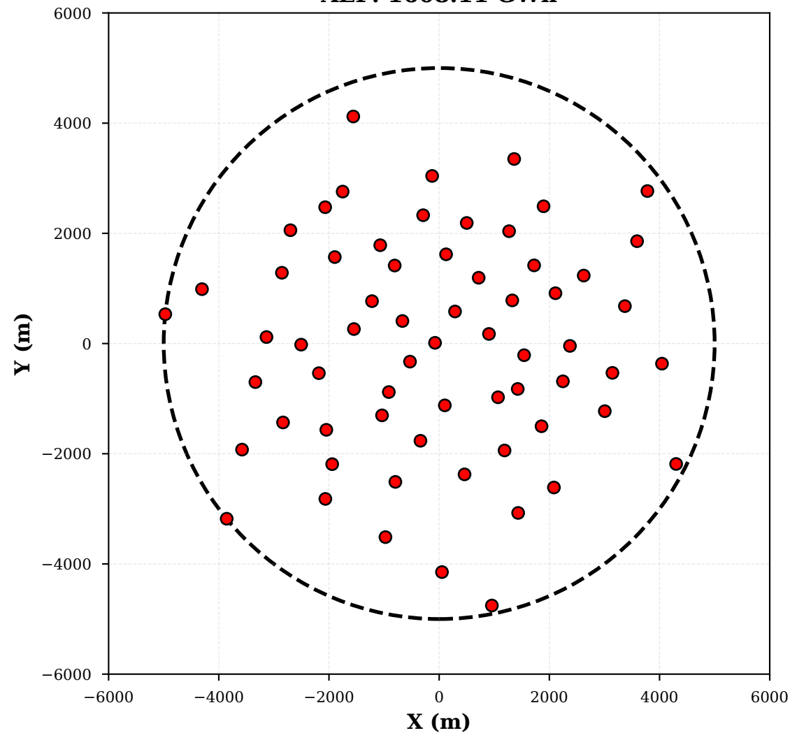
Phase 1 - Best AEP: 1608.11 GWh
