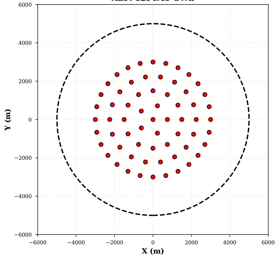
Phase 1 - Initial AEP: 1294.49 GWh
