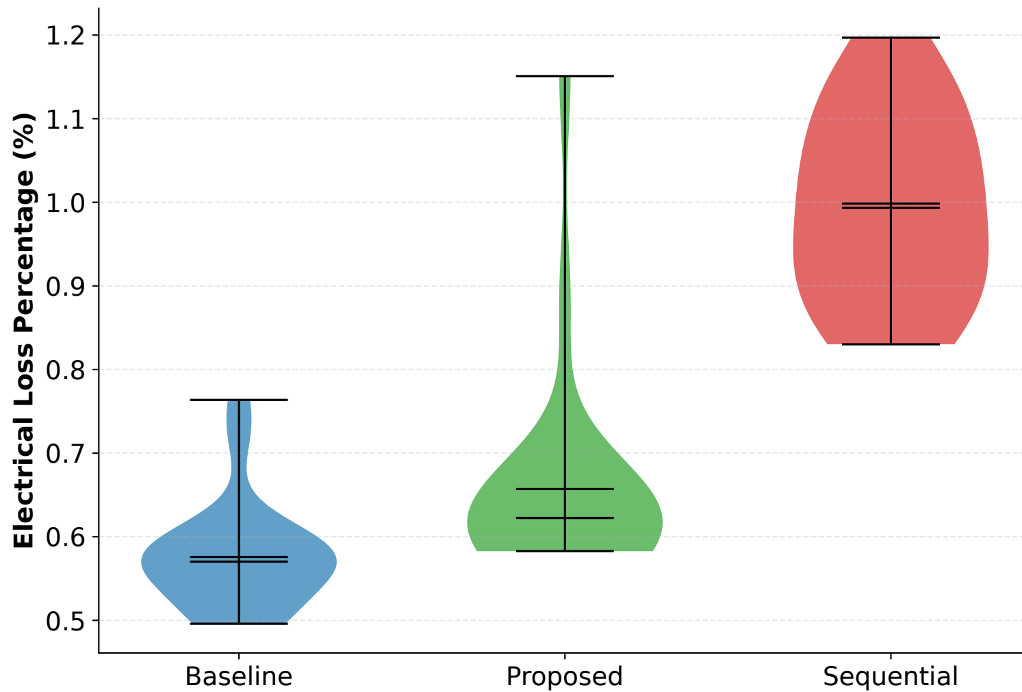
Electrical Losses
