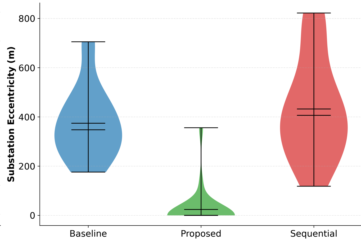
Substation Distance from Centroid
