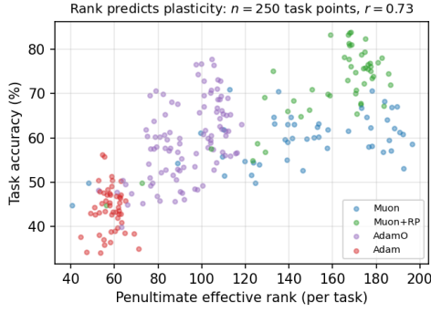
Figure 3: Effective rank predicts plasticity. Per-task accuracy vs. penultimate effective rank, one point per (method, seed, task)—250 points (CIFAR-100), r=0.73 ; within-method average +0.44 . As §7 notes, this is driven by separating the collapsed optimizer (Adam) from the rest—rank does not separate the strong optimizers from each other.
