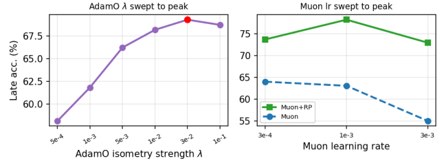
Figure 5: Both methods are tuned to their peak (CIFAR-100). Left: AdamO’s late accuracy vs. isometry strength \lambda , peaking at \lambda=3 \times 10^{-2} ; using the default \lambda understates it by up to 11 points. Right: Muon and Muon+RP vs. learning rate, peaking at 10^{-3} . Each method is reported at its own optimum, so the +9.3 gap is not a tuning artifact.
