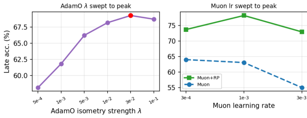
Figure 5: Both methods are tuned to their peak (CIFAR-100) . Left: AdamO's late accuracy vs. isometry strength \lambda , peaking at \lambda = 3 \times 10^{-2} ; using the default \lambda understates it by up to 11 points. Right: Muon and Muon+RP vs. learning rate, peaking at 10^{-3} . Each method is reported at its own optimum, so the +9.3 gap is not a tuning artifact.
