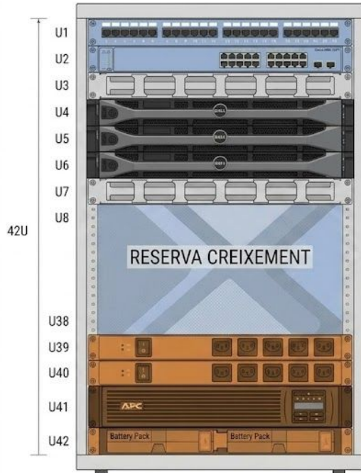
Rack 2 – Vista frontal
