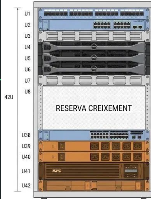
Rack 1 – Vista frontal
