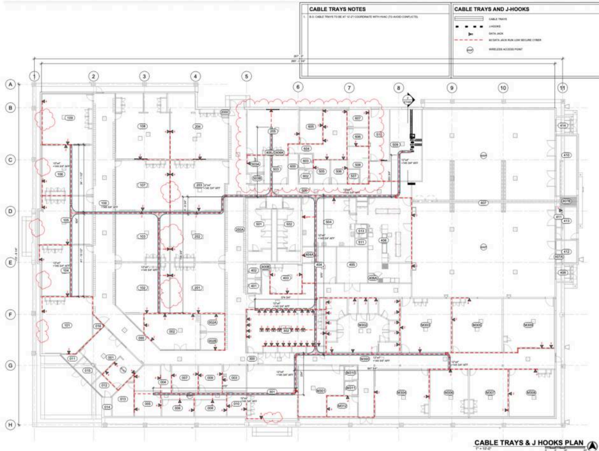
Figure 3b. Main floor Middle School building map with cable raceway trays and J hooks
