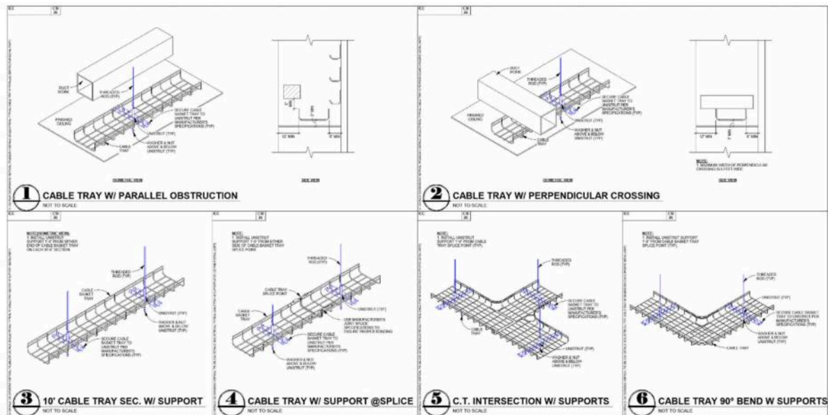
Figure 3c. Middle School Cable trays used in the main floor ceilings
