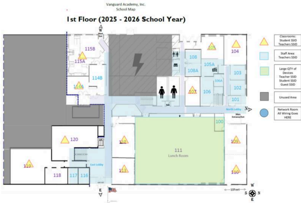
Figure 1b. 1st floor Vanguard Main building map with proposed access point placements
