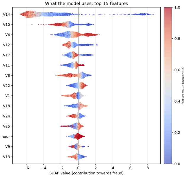
Fig. 2. SHAP values over all day-2 frauds plus 4,000 sampled legitimate rows. Every dot is one transaction, its position on the x axis is how much the feature pushed the score towards fraud, and its colour is the value of the feature, blue for low and red for high.
