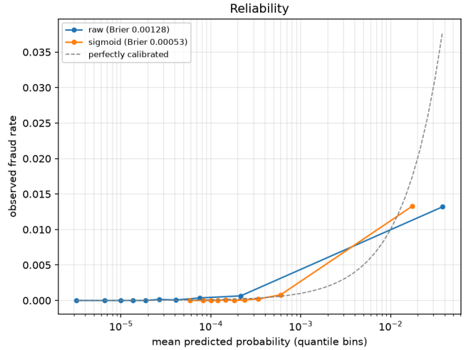
Fig. 3. Predicted probability against the fraud rate we really observed on day 2. The dashed line is what a perfect model would draw. The x axis is logarithmic because almost every score is very small.
