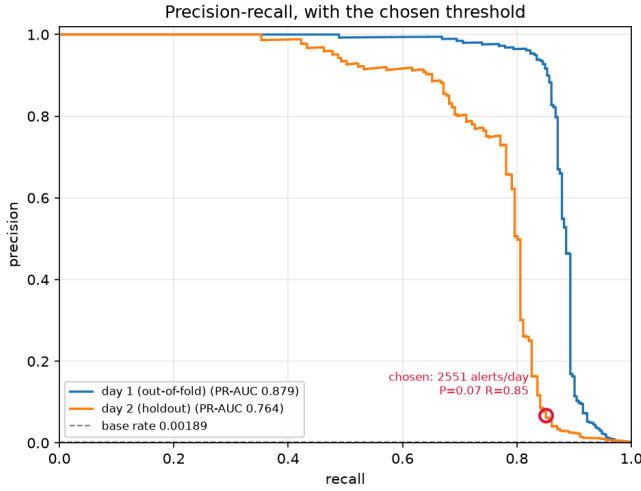
Fig. 1. Day-1 out-of-fold against the day-2 holdout. The ring is the shipped point as it landed on day 2.
