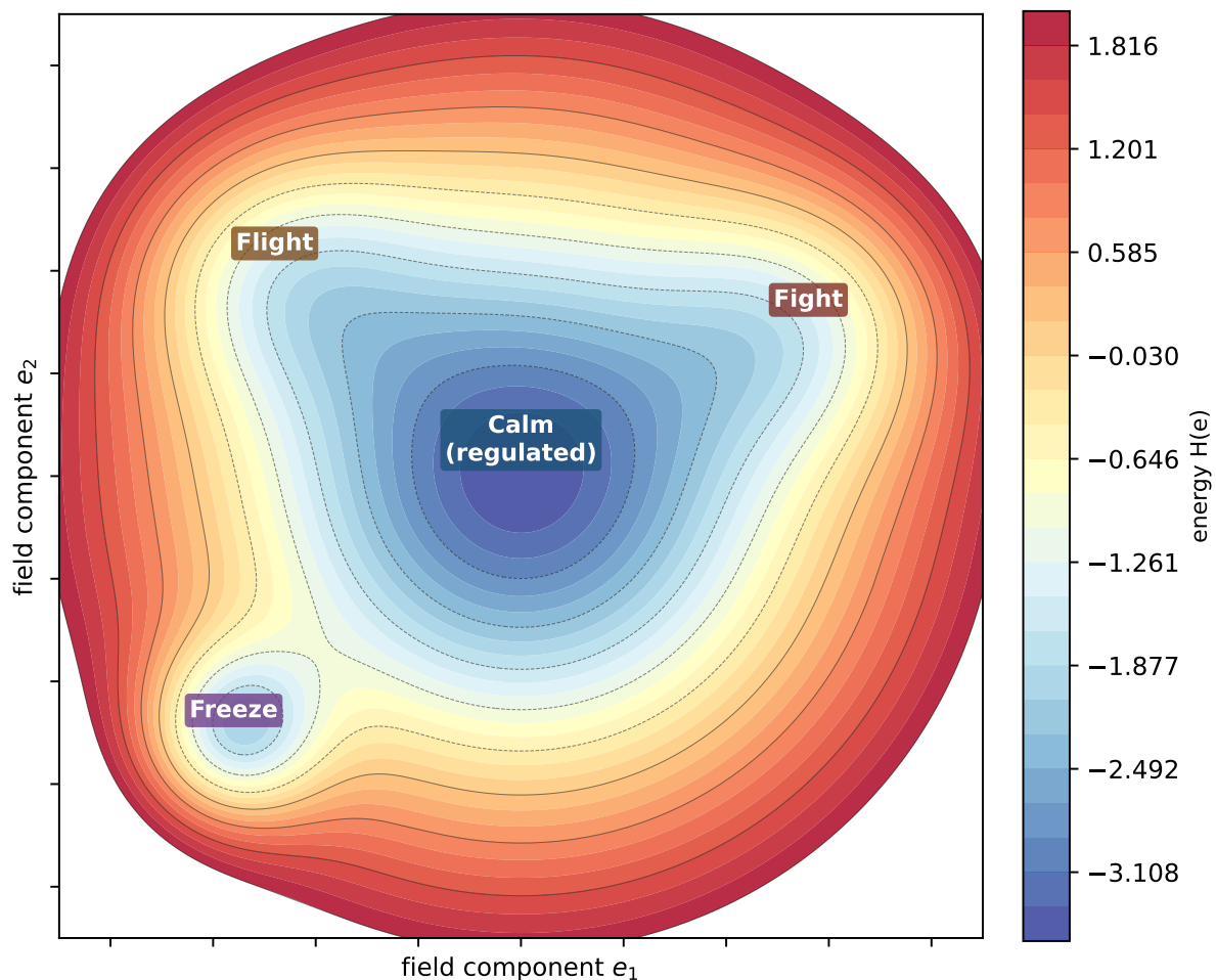
Soma-Field Energy Landscape: Four Attractor States
