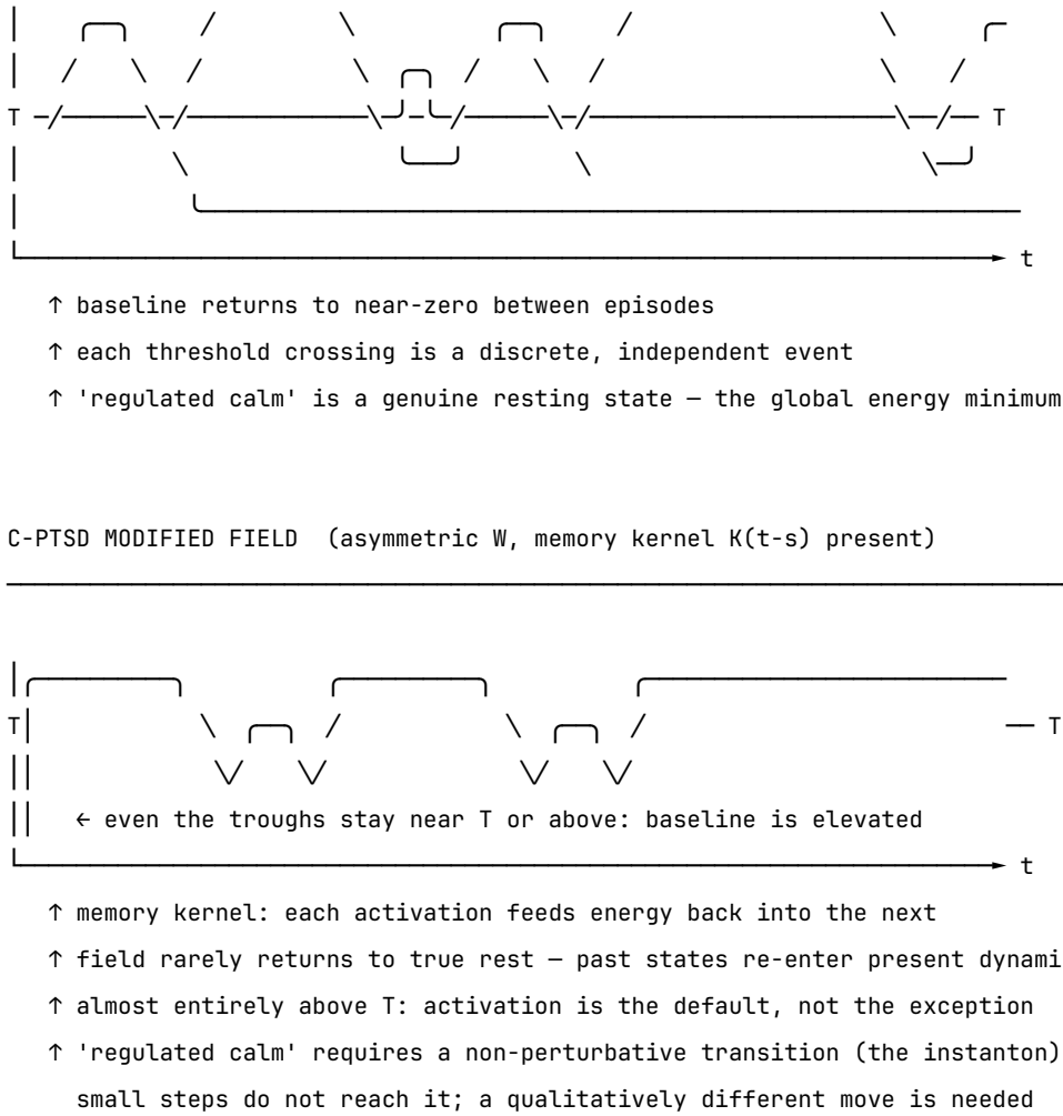
Figure 5. The same emotional field mode under two dynamic regimes. Top: regulated dynamics — the field oscillates and returns to a low baseline between episodes; conscious emotion (above T ) is episodic and resolves. Bottom: C-PTSD-modified dynamics — the memory kernel elevates the baseline so that the field rarely returns to rest; episodes bleed into one another; the system cycles rather than settles. The mathematical basis for this comparison is given in Appendix B.2.
