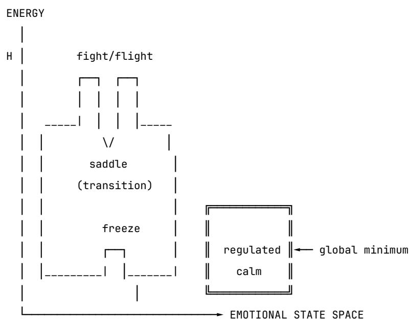
Figure 3b. Schematic energy landscape. Fight /flight are high-energy, unstable local minima. Freeze is a low-energy but isolated attractor — easy to enter, hard to escape. Regulated calm is the global energy minimum.
