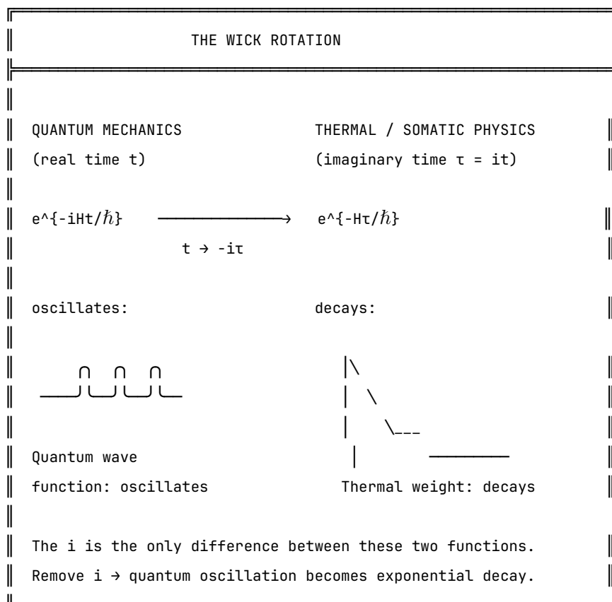
Figure 7.1. The Wick rotation. A single substitution ( t \rightarrow -i\tau ) transforms the oscillatory quantum phase factor into the real decaying exponential of thermal physics. The memory kernel K(\tau) = \sum A_k e^{-|\tau|/\tau_k} has exactly this form. The i in the quantum exponent is the only mathematical difference between a quantum field that oscillates and a trauma trace that decays.
