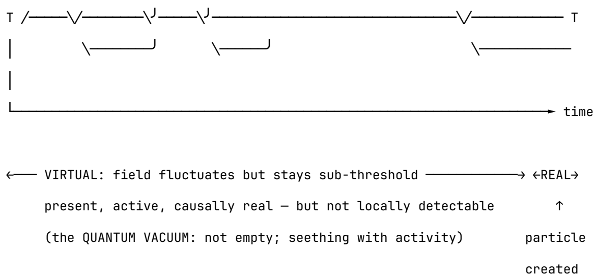
Figure o. A single field mode in quantum field theory. The field oscillates continuously. Below the detection threshold T , excitations are sub-threshold — real and causally active, but not detectable as particles. The quantum vacuum is not empty; it is a field in constant motion that never quite crosses the threshold. When the amplitude does cross T , a particle exists: a locally observable excitation. The same structure — field always present, consciousness only when threshold crossed — is the core of the Soma-Field Model.
