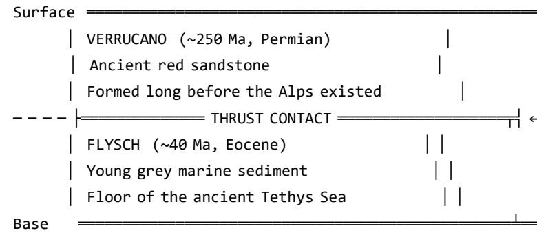
GLARUS THRUST: SCHEMATIC CROSS-SECTION (not to scale)
