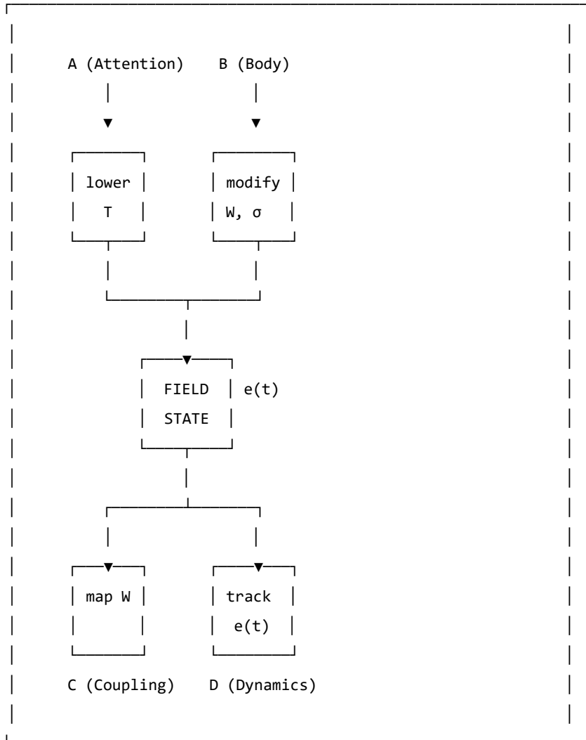
Figure 9.2. The ABCD operator circuit. Attention (A) and Body (B) are input operators that act on the field. Coupling (C) and Dynamics (D) are measurement operators that
