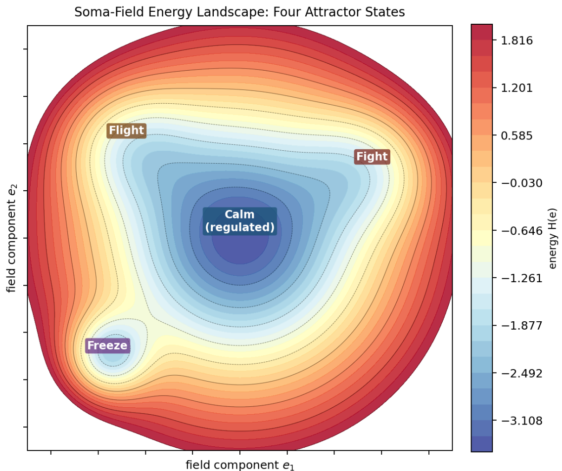
Figure 3: Figure 3.1. The emotional energy landscape (2D contour). Four attractor basins are visible: Calm (wide, deepest — the global minimum of a regulated nervous system), Freeze (narrow and very deep — easy to fall into, hard to leave), Fight and Flight (intermediate depth). The system rolls downhill to the nearest basin; the depth controls escape difficulty and the width controls resilience to perturbation. Author's original figure.
