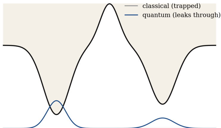
F13.2 Tunnelling through an energy barrier
