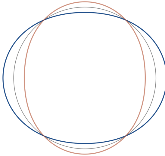
F5.1 Earth \text{oS}_2 — the 'football' free oscillation period \approx 54 minutes
