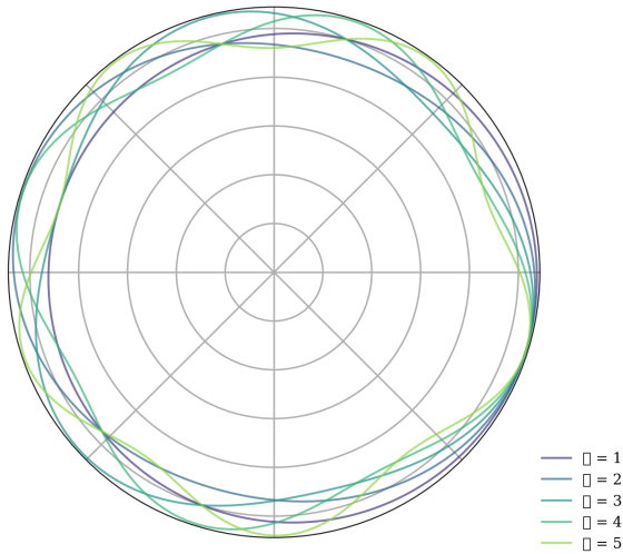
F4.2 Solar p-mode oscillations (spherical harmonics \ell = 1..5 )
