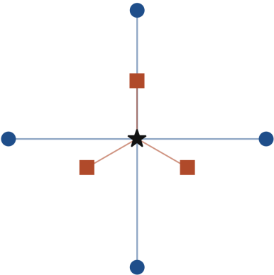
F15.2 G_2 holonomy — seven internal directions of feeling
