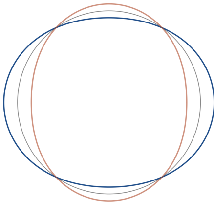
F5.1 Earth \alpha_2 — the ‘football’ free oscillation period \approx 54 minutes
