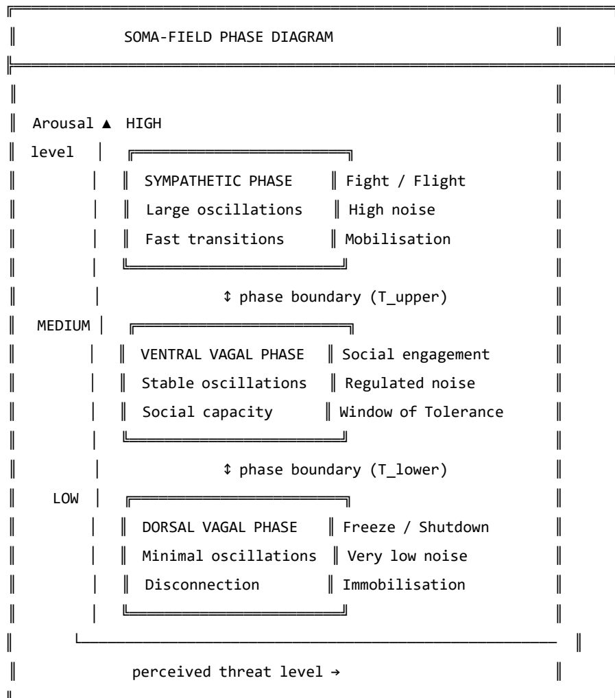
Figure 8.1. The nervous system as a phase diagram. Three distinct phases correspond to the three polyvagal states. Phase boundaries ( T_{upper} and T_{lower} ) mark the transitions. For a regulated nervous system, most experience occurs in the ventral
