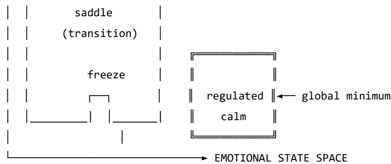
Figure 2. The emotional energy landscape. The freeze state is not high-energy — it is isolated. This distinction matters enormously. The author is aware of this from personal experience, over many years, and from the other side.
