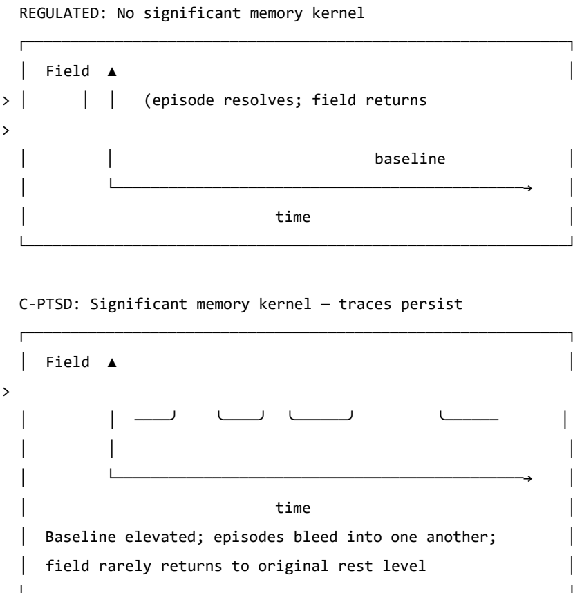
Figure 5.1. The effect of the trauma memory kernel on field dynamics. In a regulated system (top), a field activation episode resolves and the field returns to a low resting level. In the C-PTSD-modified system (bottom), the memory kernel elevates the baseline between episodes, so that subsequent episodes begin from a higher resting activation. Over time, the field cycles at an elevated level without returning to rest.
