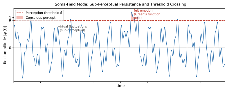
Figure 10. Continuous soma-field activity (blue) with a single threshold-crossing event. The field is always active; conscious experience (shaded) arises
