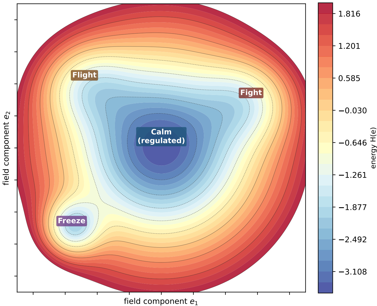
Soma-Field Energy Landscape: Four Attractor States
